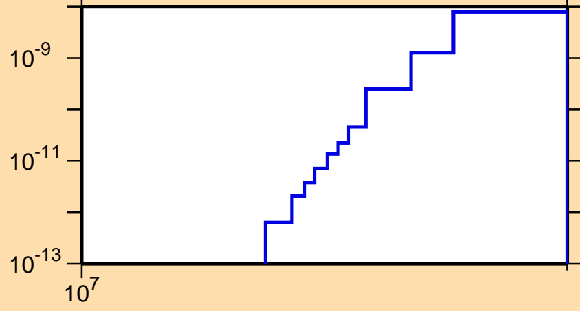
\sigma vs. E for ^{224}\text{Fr}(n,3n\alpha)
