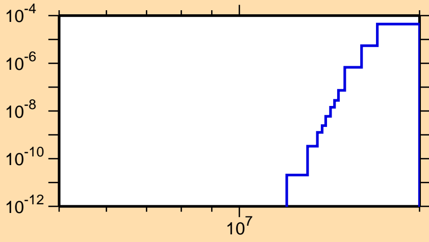
\sigma vs. E for ^{224}\text{Fr}(n,nt)
