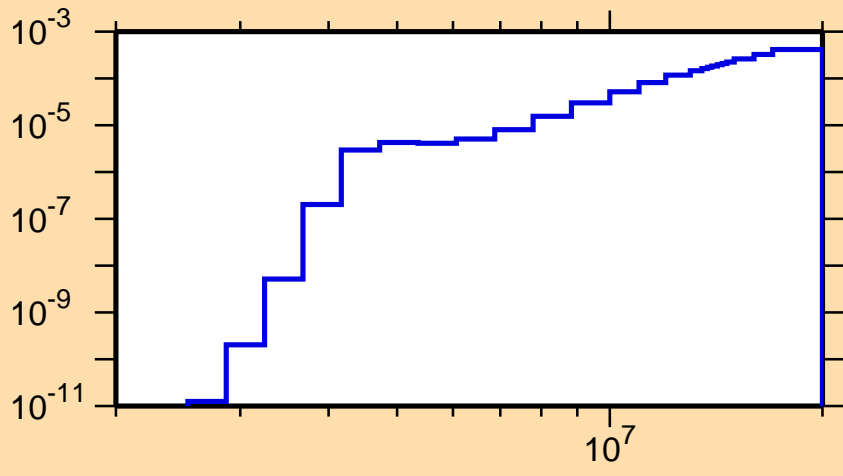
\sigma vs. E for ^{224}\text{Fr}(n,f)
