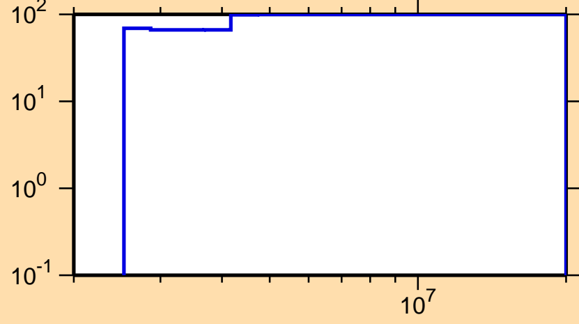
\Delta\sigma/\sigma vs. E for ^{224}\text{Fr}(n,\gamma)
