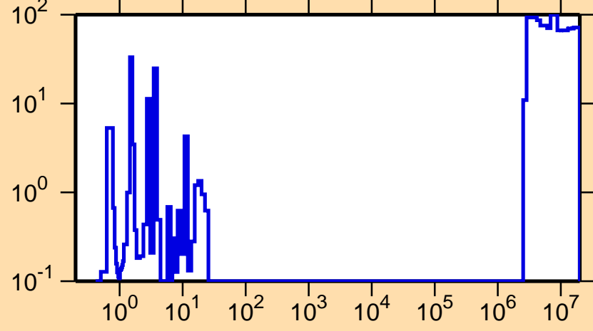
\Delta\sigma/\sigma vs. E for ^{224}\text{Fr}(n,f)
