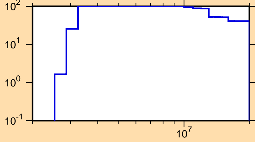
\Delta\sigma/\sigma vs. E for ^{224}\text{Fr}(n,p)
