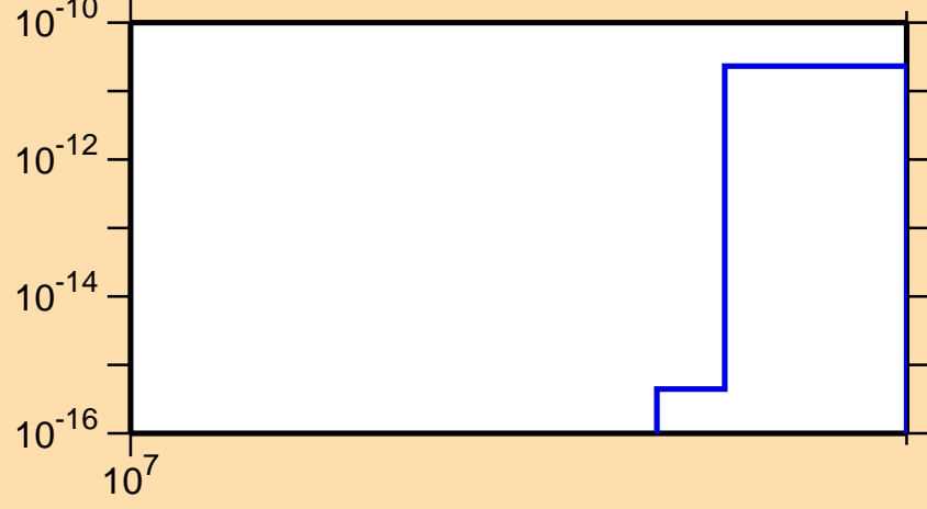
\sigma vs. E for ^{224}\text{Fr} (mt 11)
