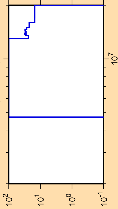
\Delta\sigma/\sigma vs. E for ^{224}\text{Fr}(n,n\text{cont.})
