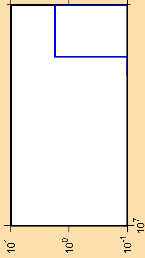
\Delta\sigma/\sigma vs. E for ^{224}\text{Fr} (mt 42)
