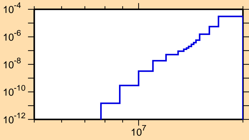
\sigma vs. E for ^{224}\text{Fr}(n,2n\alpha)
