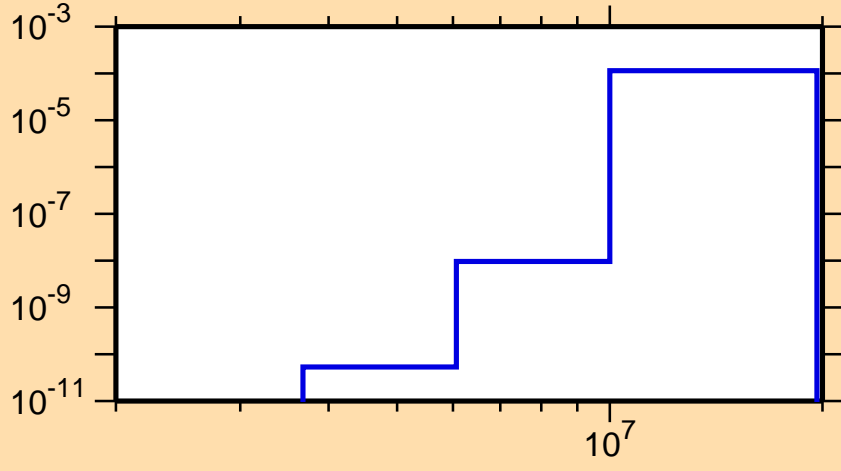
\sigma vs. E for ^{224}\text{Fr}(n,n\alpha)
