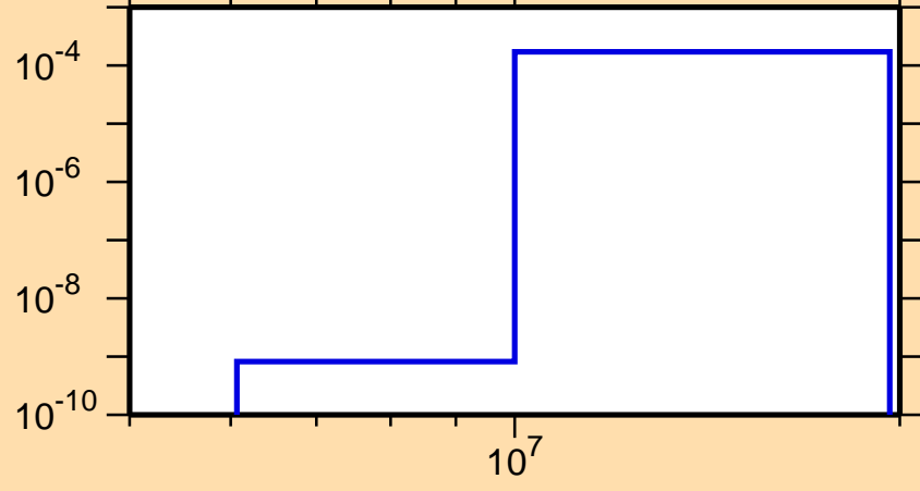
\sigma vs. E for ^{224}\text{Fr}(n,t)
