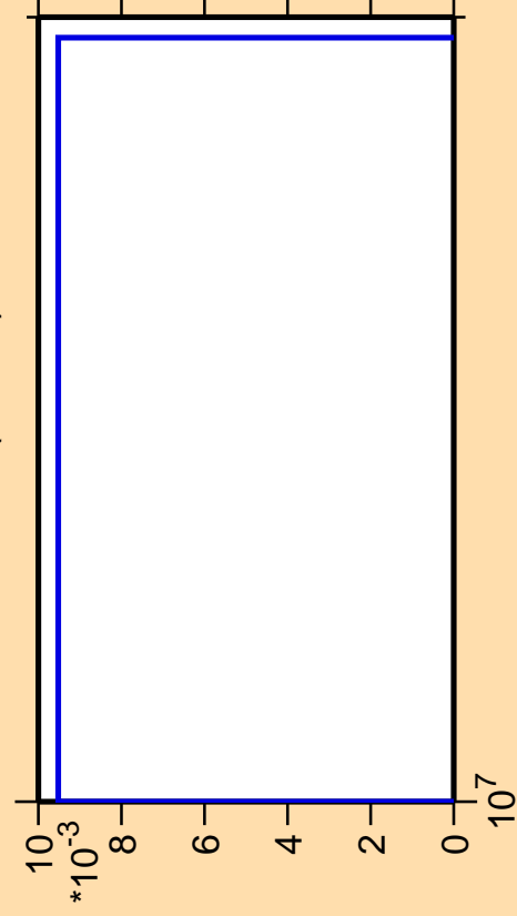
\Delta\sigma/\sigma vs. E for ^{224}\text{Fr}(\text{mt } 42)
