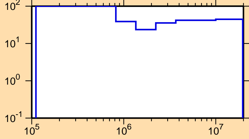
\Delta\sigma/\sigma vs. E for ^{224}\text{Fr}(n,\text{nonel.})
