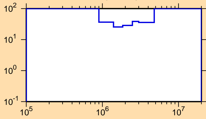
\Delta\sigma/\sigma vs. E for ^{224}\text{Fr}(n,\text{inel.})
