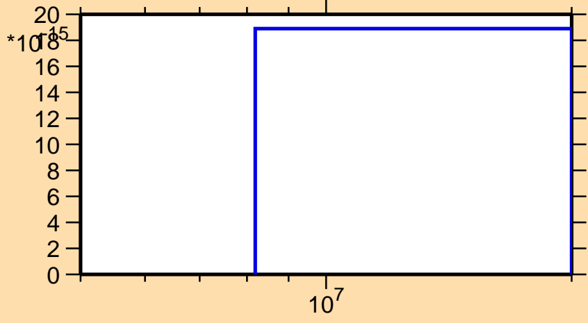
\sigma vs. E for ^{224}\text{Fr}(\text{mt } 42)
