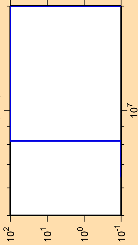
\Delta\sigma/\sigma vs. E for ^{224}\text{Fr}(n,nt)
