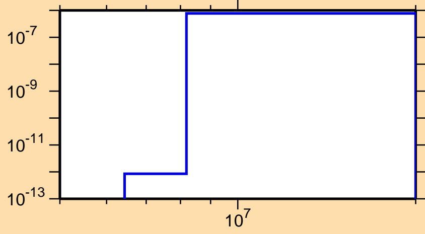
\sigma vs. E for ^{224}\text{Fr}(n,2n\alpha)
