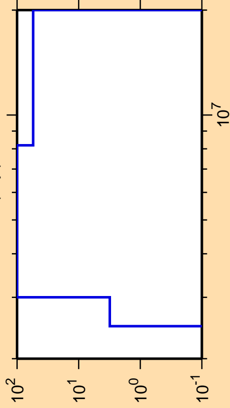
\Delta\sigma/\sigma vs. E for ^{224}\text{Fr}(n,p)
