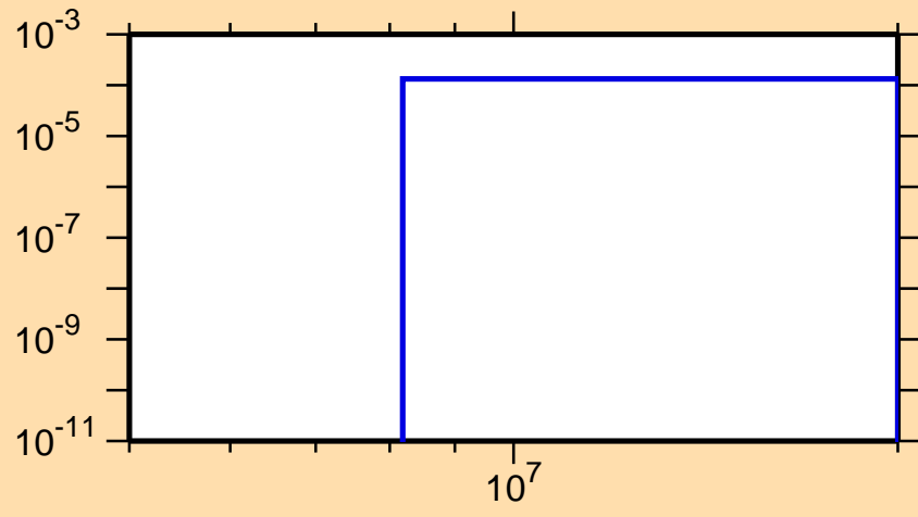
\sigma vs. E for ^{224}\text{Fr}(n,d)
