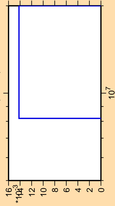
\Delta\sigma/\sigma vs. E for ^{224}\text{Fr}(\text{mt } 42)
