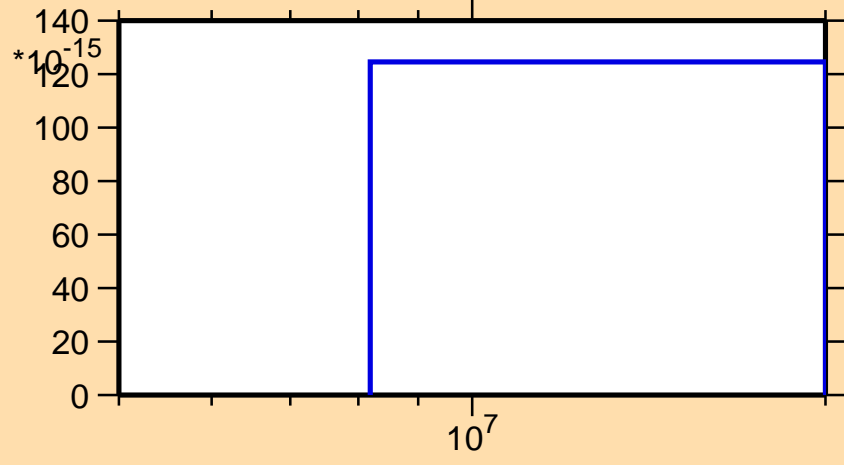
\sigma vs. E for ^{224}\text{Fr}(n,\text{He}3)
