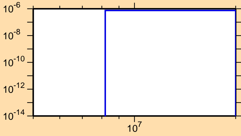
\sigma vs. E for ^{224}\text{Fr}(n,\text{nd})
