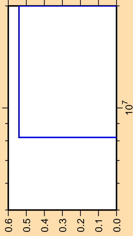
\Delta\sigma/\sigma vs. E for ^{224}\text{Fr}(\text{mt } 11)
