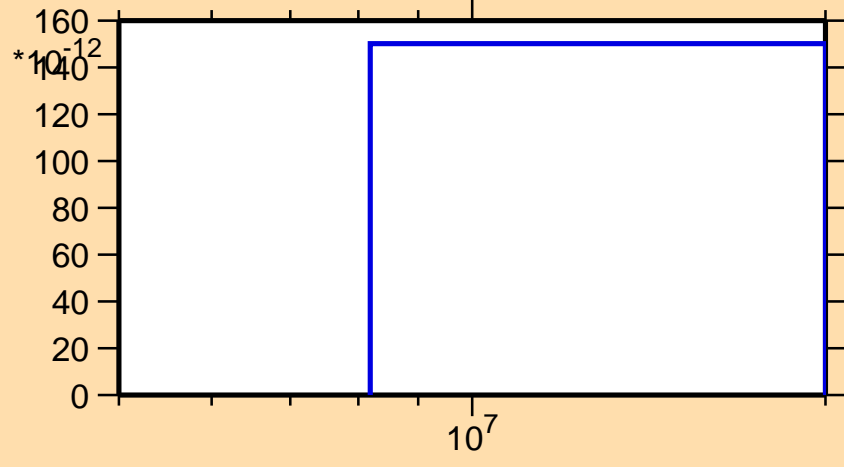
\sigma vs. E for ^{224}\text{Fr}(n,3n\alpha)
