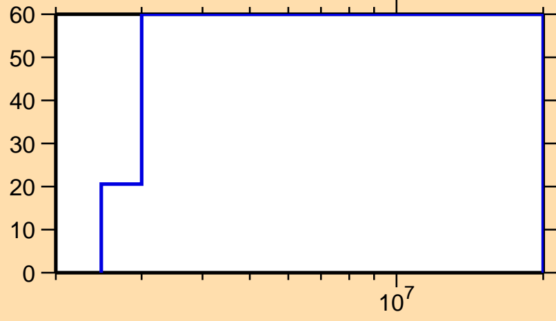
\Delta\sigma/\sigma vs. E for ^{224}\text{Fr}(n,f)
