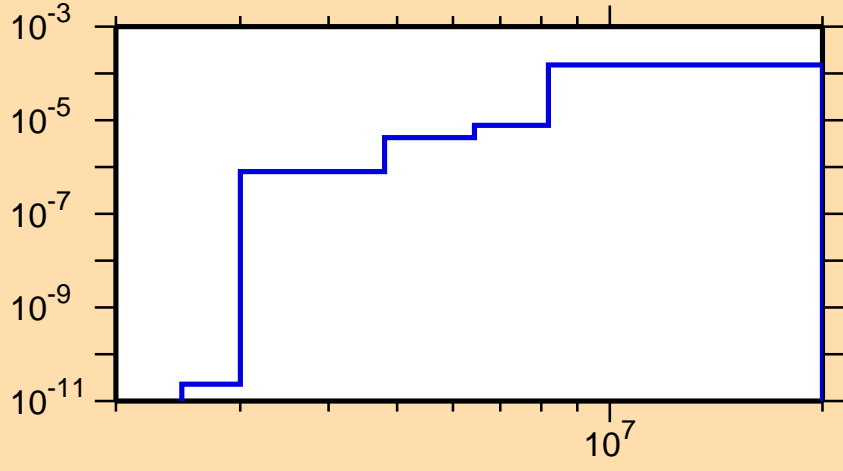
\sigma vs. E for ^{224}\text{Fr}(n,f)
