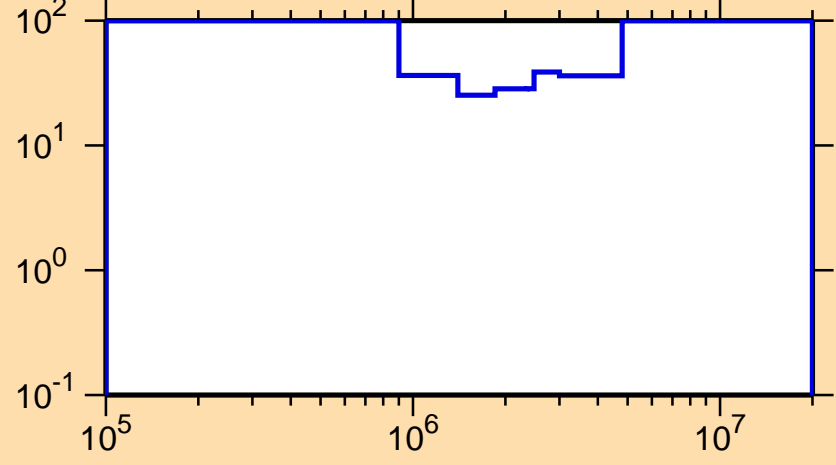
\Delta\sigma/\sigma vs. E for ^{224}\text{Fr}(n,n\text{cont.})
