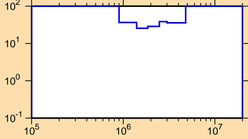
\Delta\sigma/\sigma vs. E for ^{224}\text{Fr}(n,\text{inel.})
