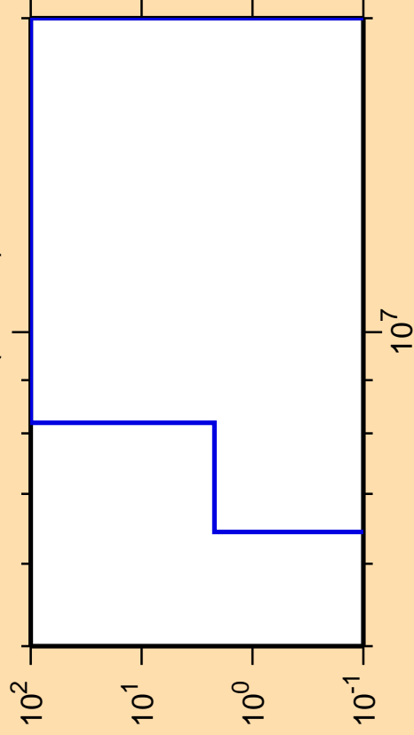
\Delta\sigma/\sigma vs. E for ^{224}\text{Fr}(n,2n\alpha)
