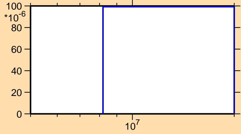
\sigma vs. E for ^{224}\text{Fr}(n,np)
