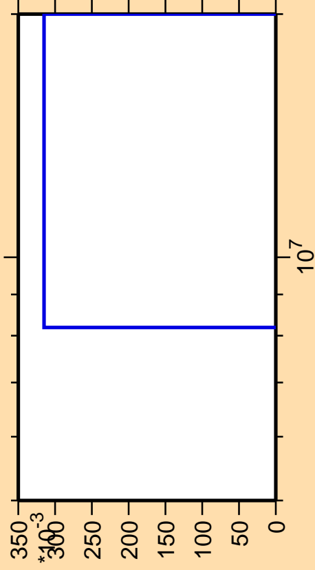
\Delta\sigma/\sigma vs. E for ^{224}\text{Fr}(n,\text{He}3)
