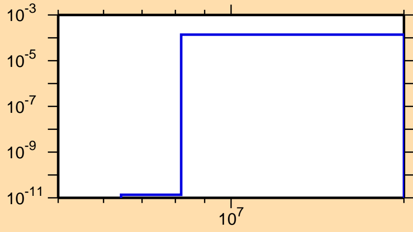
\sigma vs. E for ^{224}\text{Fr}(n,t)
