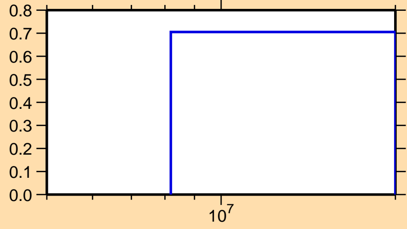
\sigma vs. E for ^{224}\text{Fr}(n,3n)
