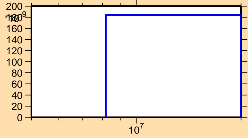
\sigma vs. E for ^{224}\text{Fr}(n,2np)
