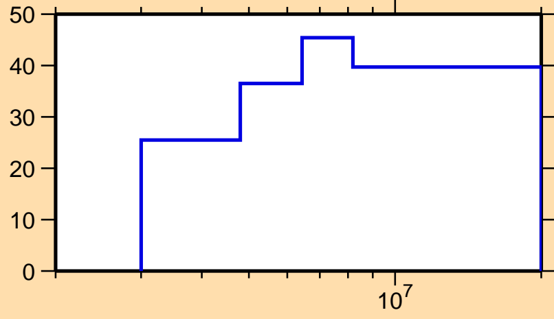
\Delta\sigma/\sigma vs. E for ^{224}\text{Fr}(n,\text{tot.})
