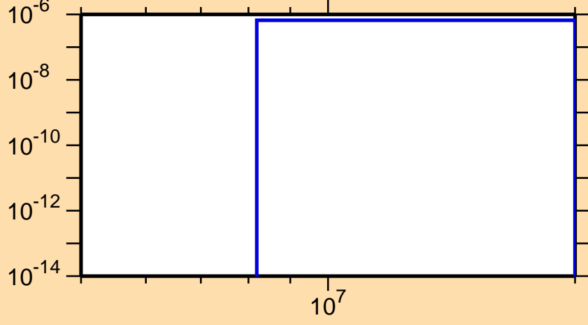
\sigma vs. E for ^{224}\text{Fr}(n,nt)
