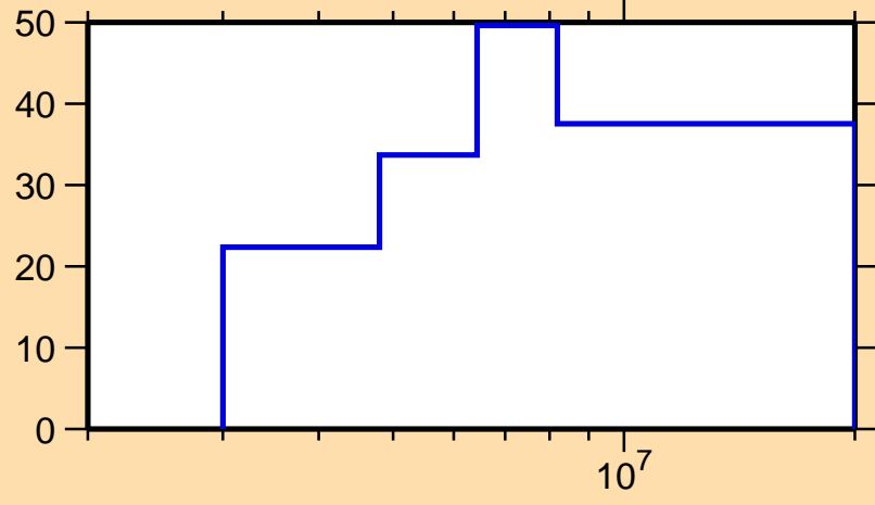
\Delta\sigma/\sigma vs. E for ^{224}\text{Fr}(n,\text{el.})
