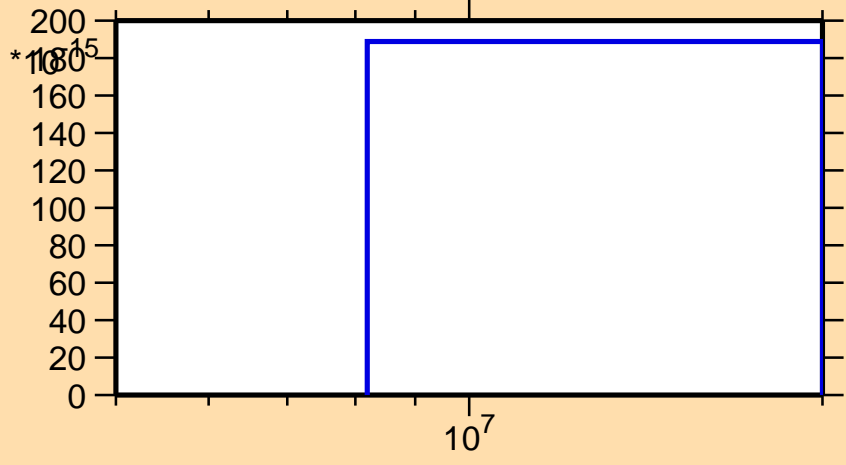
\sigma vs. E for ^{224}\text{Fr}(\text{mt } 11)
