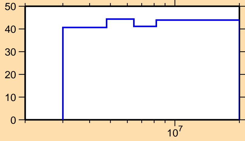
\Delta\sigma/\sigma vs. E for ^{224}\text{Fr}(n,\text{nonel.})
