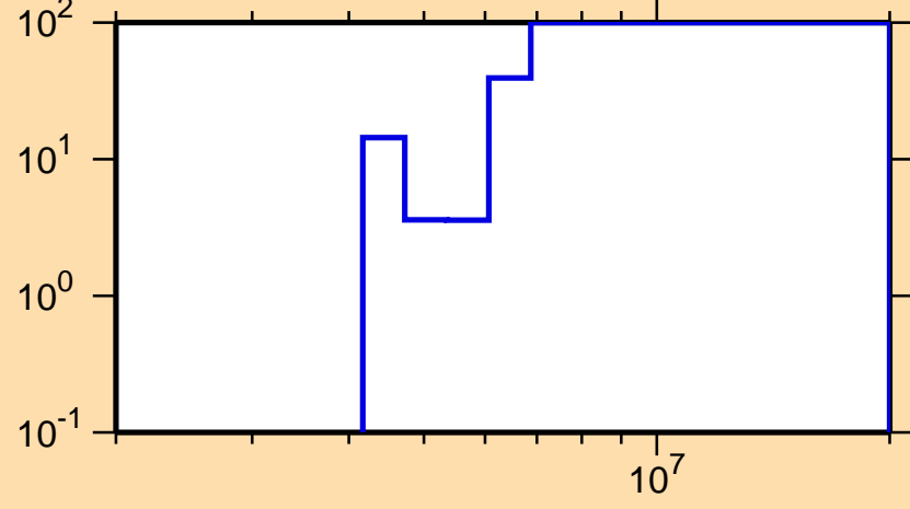
\Delta\sigma/\sigma vs. E for ^{225}\text{Fr}(n,\text{inel.})
