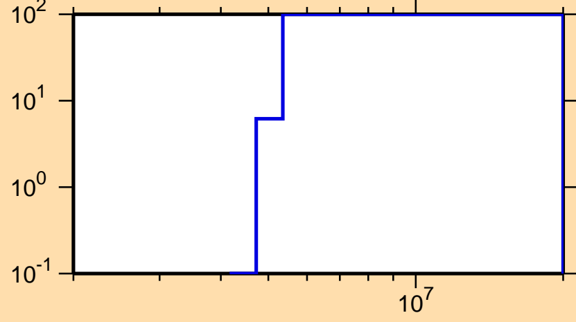
\Delta\sigma/\sigma vs. E for ^{225}\text{Fr}(n,p)
