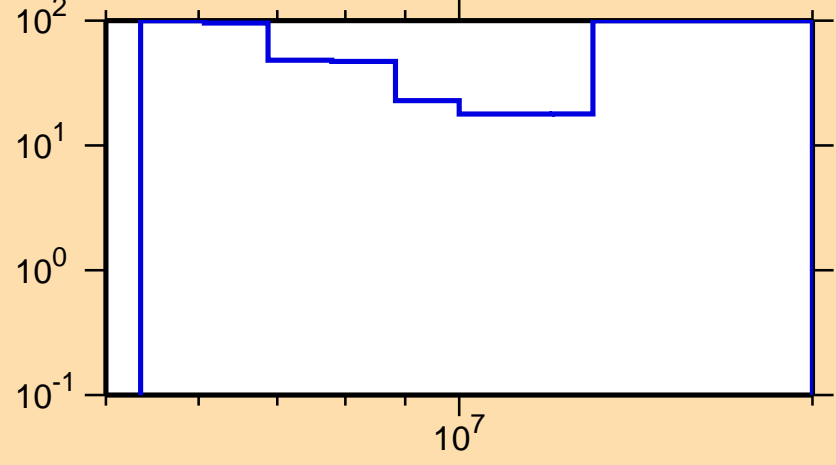
\Delta\sigma/\sigma vs. E for ^{225}\text{Fr}(n,2n)
