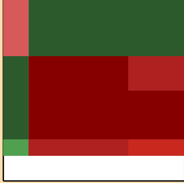
\Delta\sigma/\sigma vs. E for ^{225}\text{Fr}(n,\text{inel.})
