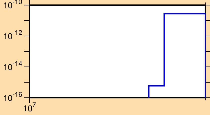
\sigma vs. E for ^{225}\text{Fr} (mt 11)
