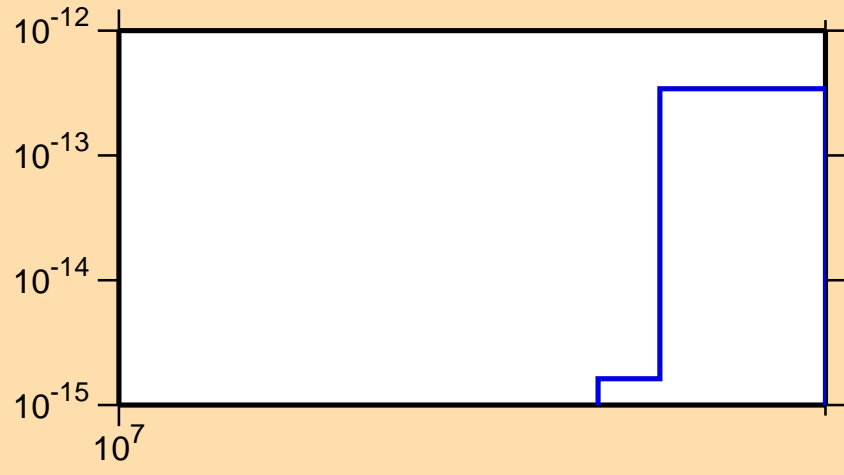
\sigma vs. E for ^{225}\text{Fr}(n,\text{He}3)
