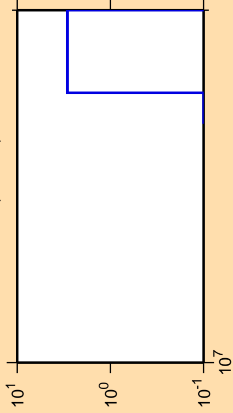
\Delta\sigma/\sigma vs. E for ^{225}\text{Fr}(n,\text{He}3)
