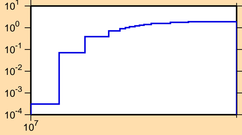
\sigma vs. E for ^{225}\text{Fr}(n,3n)
