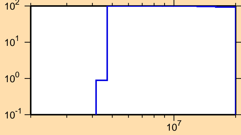
\Delta\sigma/\sigma vs. E for ^{225}\text{Fr}(n,f)
