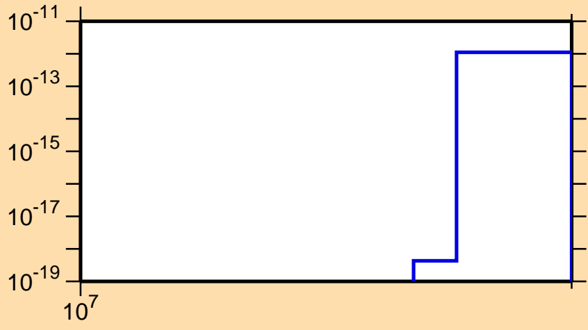
\sigma vs. E for ^{225}\text{Fr} (mt 42)
