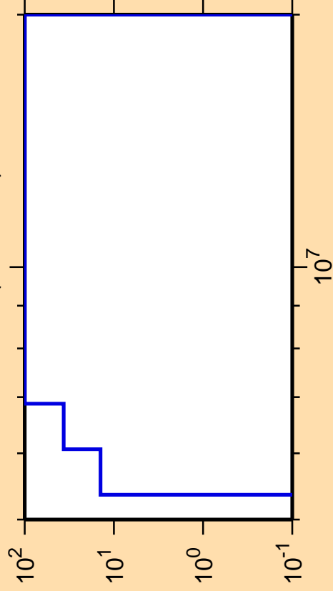
\Delta\sigma/\sigma vs. E for ^{225}\text{Fr}(n,n\text{cont.})
