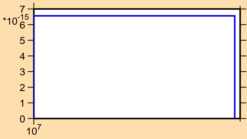
\sigma vs. E for ^{225}\text{Fr}(\text{mt } 42)
