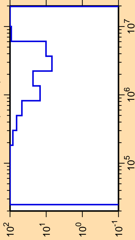
\Delta\sigma/\sigma vs. E for ^{225}\text{Fr}(n,\text{inel.})
