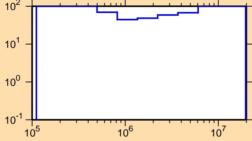
\Delta\sigma/\sigma vs. E for ^{226}\text{Fr}(n,n\text{cont.})
