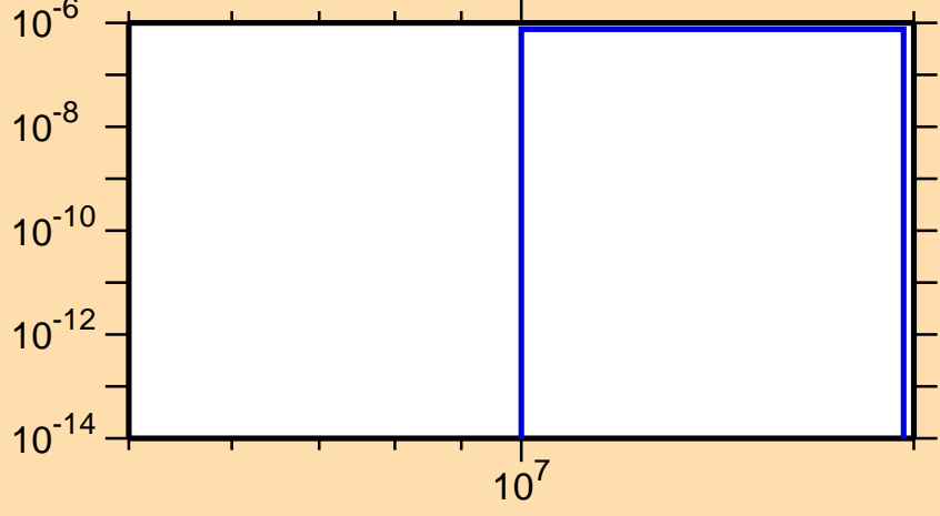
\sigma vs. E for ^{226}\text{Fr}(n,\text{nd})
