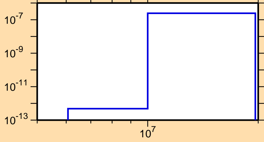
\sigma vs. E for ^{226}\text{Fr}(n,2n\alpha)
