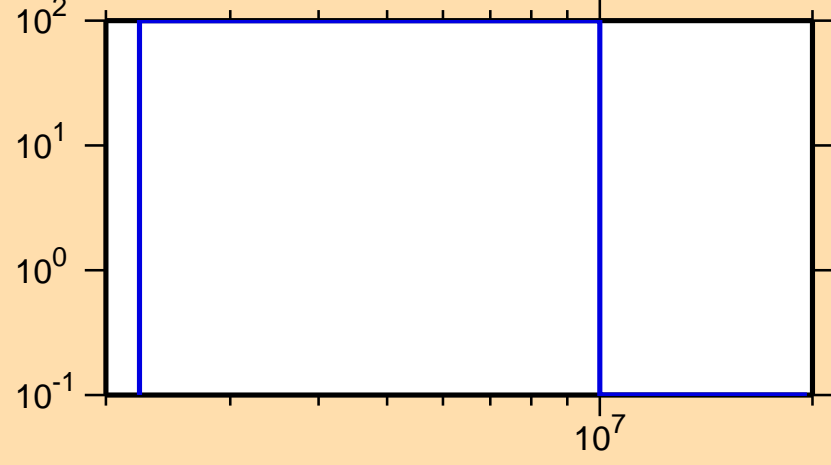
\Delta\sigma/\sigma vs. E for ^{226}\text{Fr}(n,n_1)
