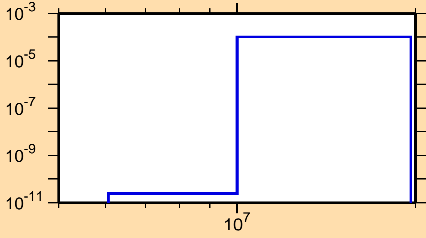
\sigma vs. E for ^{226}\text{Fr}(n,d)
