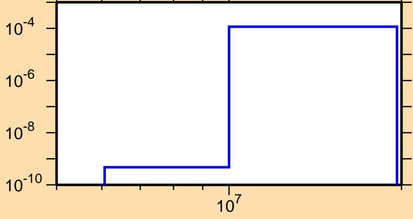
\sigma vs. E for ^{226}\text{Fr}(n,t)
