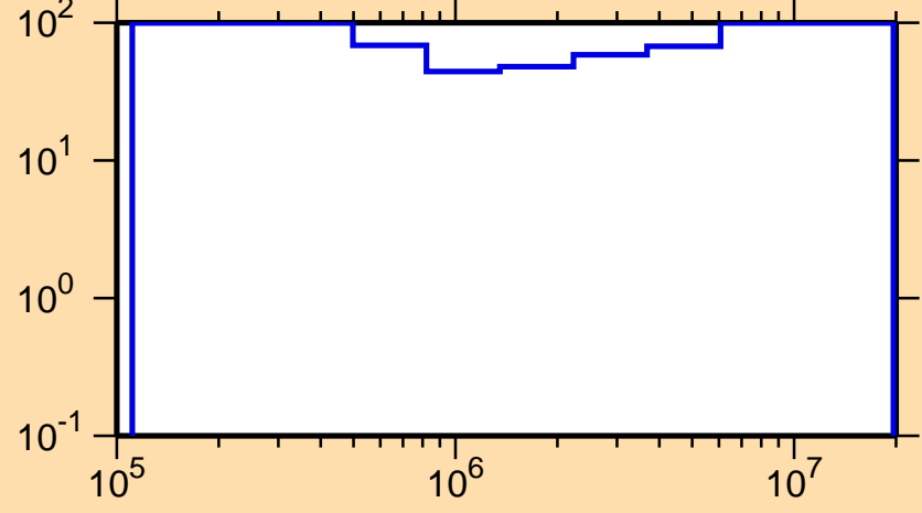
\Delta\sigma/\sigma vs. E for ^{226}\text{Fr}(n,\text{inel.})
