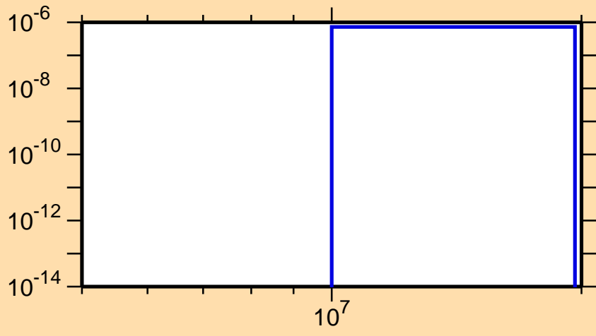
\sigma vs. E for ^{226}\text{Fr}(n,nt)
