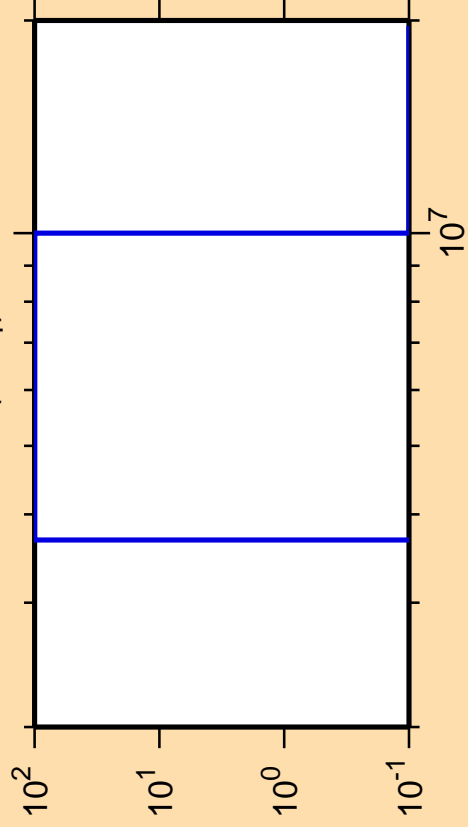
\Delta\sigma/\sigma vs. E for ^{226}\text{Fr}(n,n_1)
