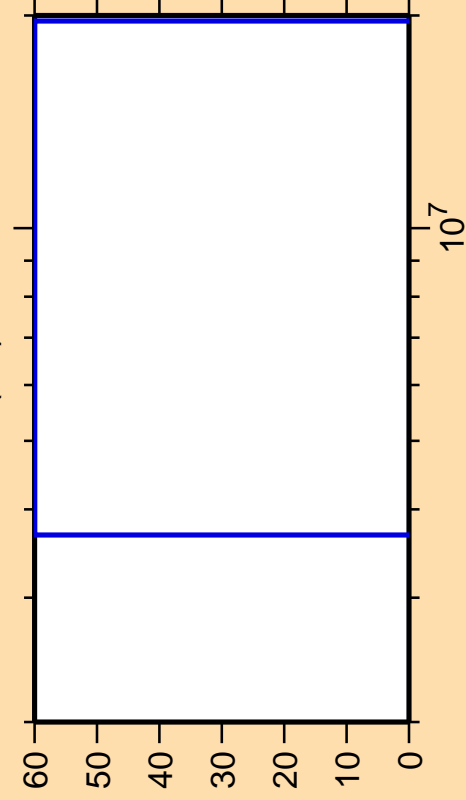
\Delta\sigma/\sigma vs. E for ^{226}\text{Fr}(n,f)
