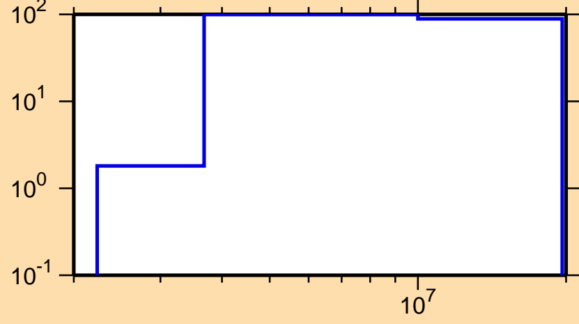
\Delta\sigma/\sigma vs. E for ^{226}\text{Fr}(n,p)
