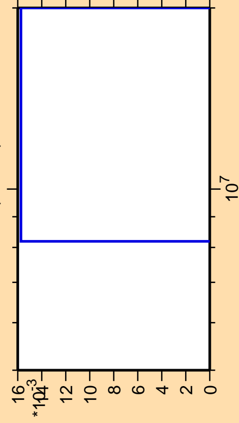
\Delta\sigma/\sigma vs. E for ^{226}\text{Fr}(\text{mt } 42)
