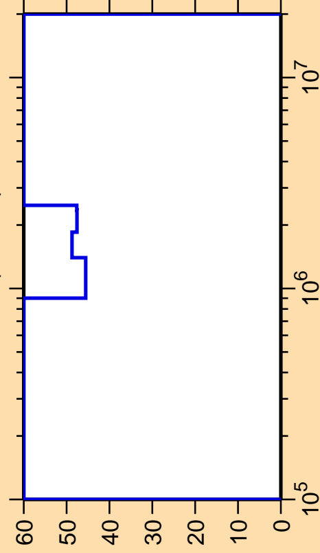
\Delta\sigma/\sigma vs. E for ^{226}\text{Fr}(n,\text{inel.})
