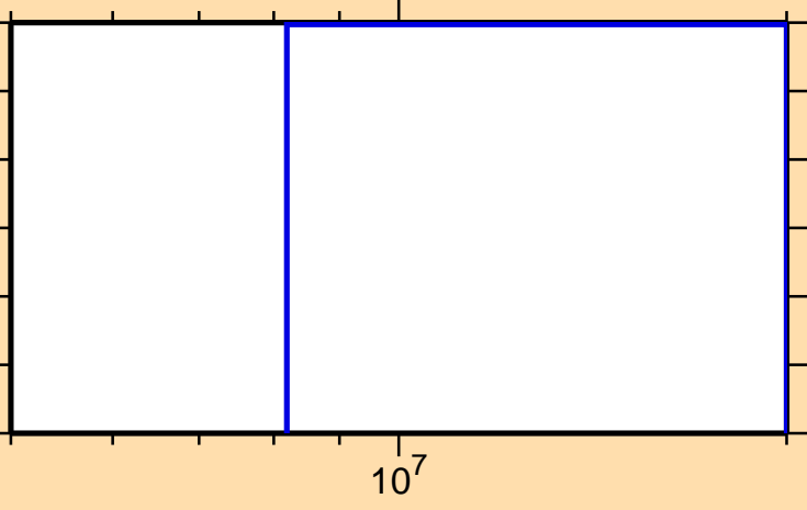
\sigma vs. E for ^{226}\text{Fr}(n,nt)
