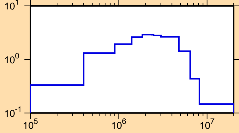
\sigma vs. E for ^{226}\text{Fr}(n,\text{inel.})
