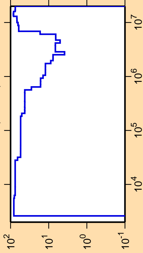
\Delta\sigma/\sigma vs. E for ^{227}\text{Fr}(n,\text{inel.})
