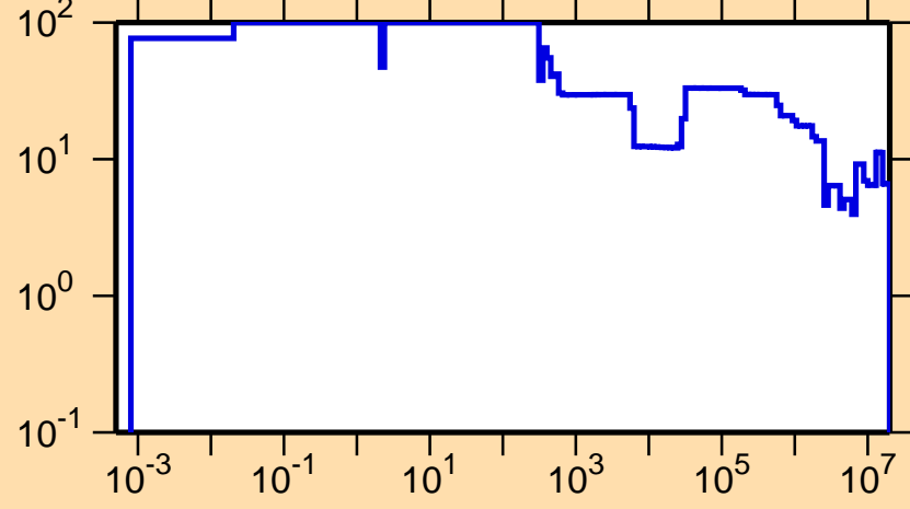
\Delta\sigma/\sigma vs. E for ^{227}\text{Fr}(n,\text{nonel.})
