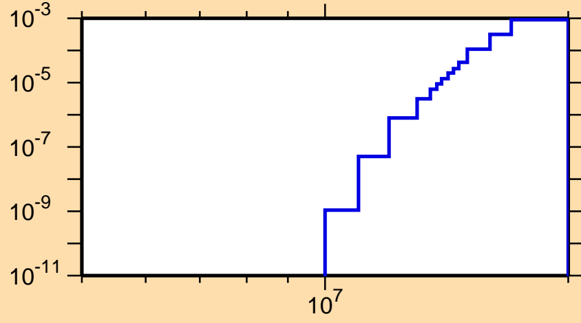
\sigma vs. E for ^{227}\text{Fr}(n,np)
