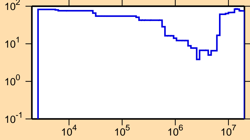
\Delta\sigma/\sigma vs. E for ^{227}\text{Fr}(n,\text{inel.})
