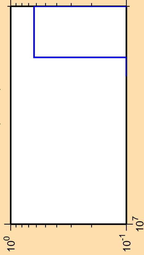
\Delta\sigma/\sigma vs. E for ^{227}\text{Fr}(\text{mt } 42)
