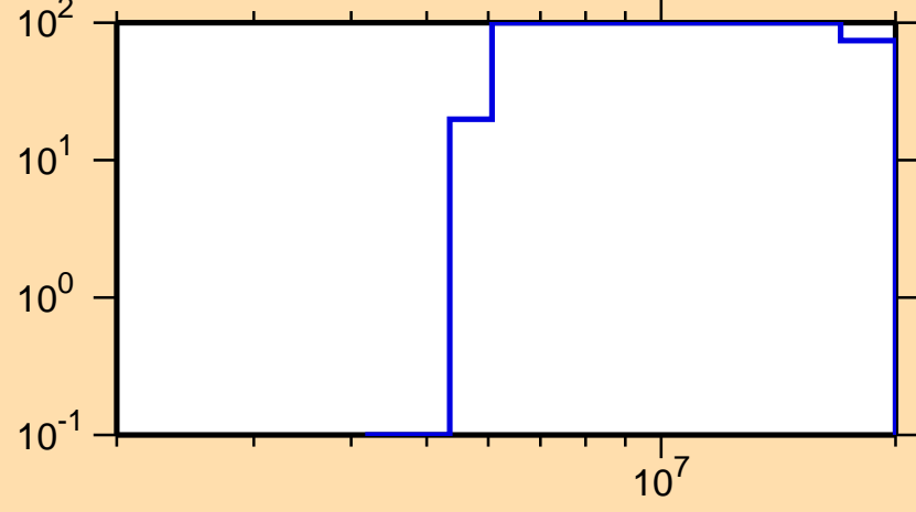
\Delta\sigma/\sigma vs. E for ^{227}\text{Fr}(n,p)
