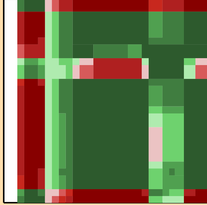
\Delta\sigma/\sigma vs. E for ^{227}\text{Fr}(n,n\text{cont.})
