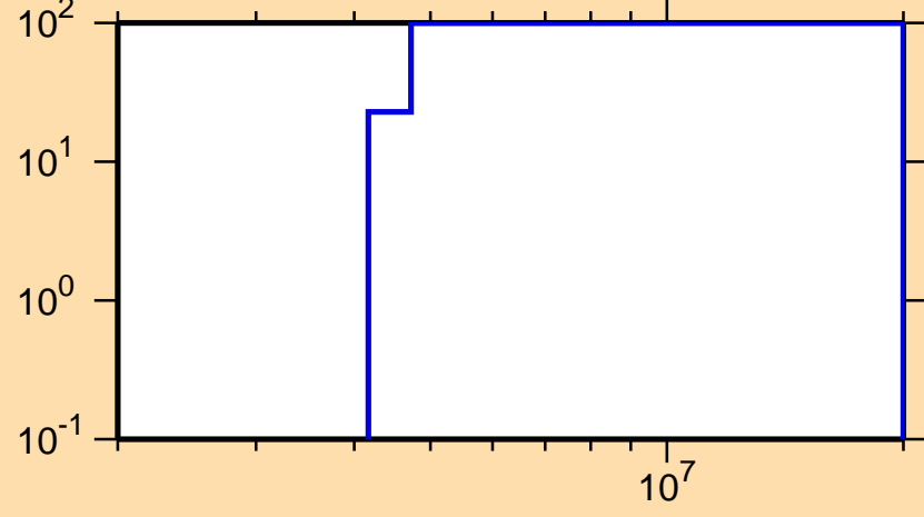
\Delta\sigma/\sigma vs. E for ^{227}\text{Fr}(n,f)
