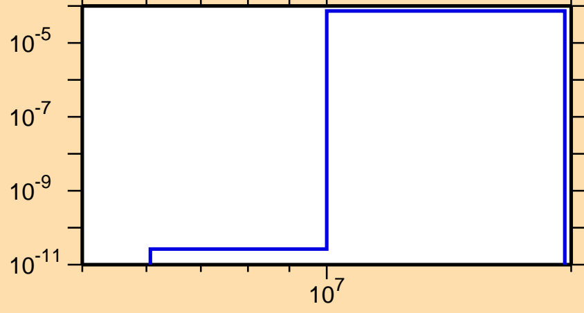
\sigma vs. E for ^{227}\text{Fr}(n,d)
