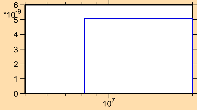
\sigma vs. E for ^{227}\text{Fr}(n,2n\alpha)
