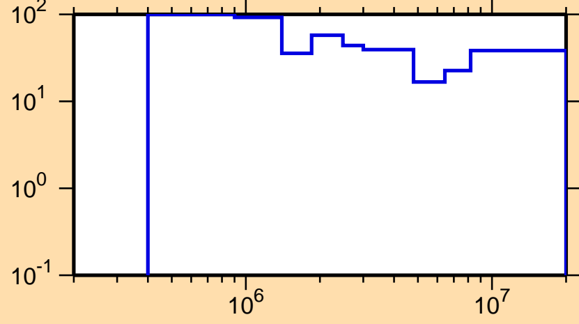
\Delta\sigma/\sigma vs. E for ^{227}\text{Fr}(n,n\text{cont.})
