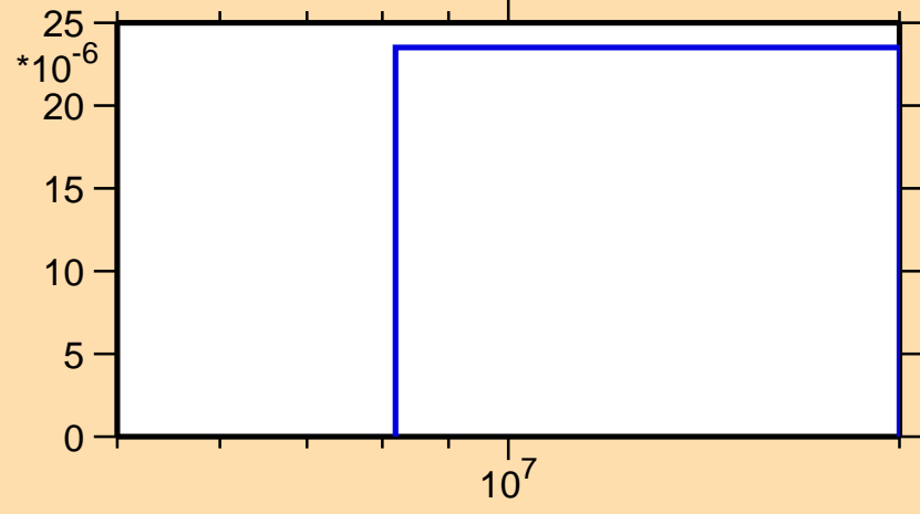
\sigma vs. E for ^{227}\text{Fr}(n,t)
