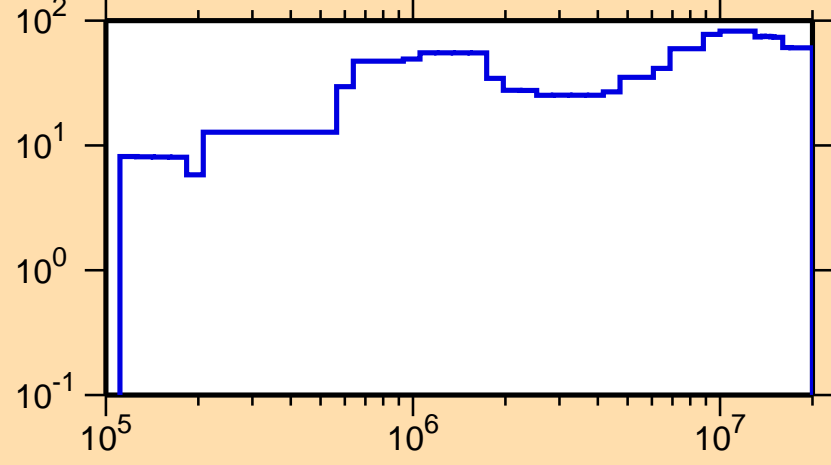
\Delta\sigma/\sigma vs. E for ^{228}\text{Fr}(n,\text{el.})
