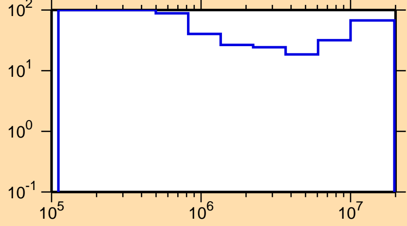
\Delta\sigma/\sigma vs. E for ^{228}\text{Fr}(n,\text{inel.})
