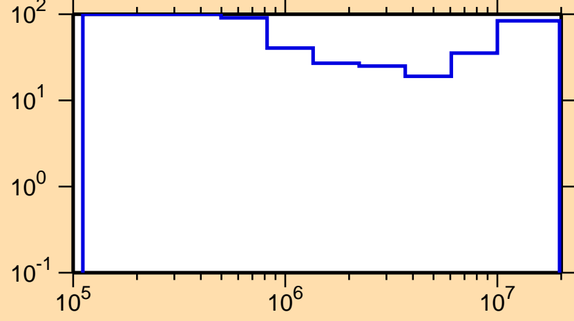
\Delta\sigma/\sigma vs. E for ^{228}\text{Fr}(n,n\text{cont.})
