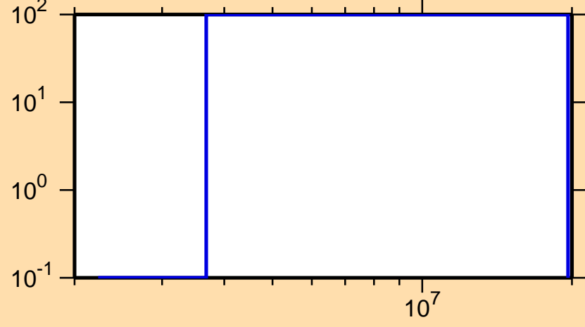
\Delta\sigma/\sigma vs. E for ^{228}\text{Fr}(n,p)
