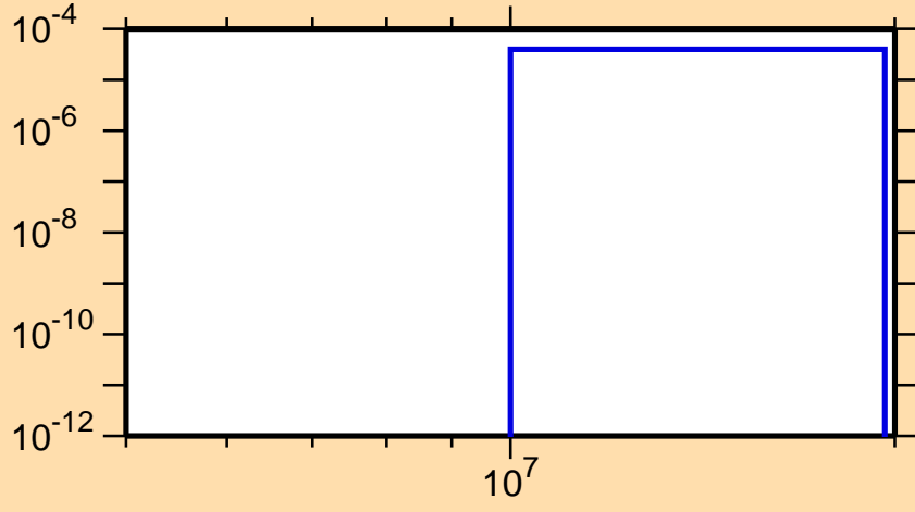
\sigma vs. E for ^{228}\text{Fr}(n,np)
