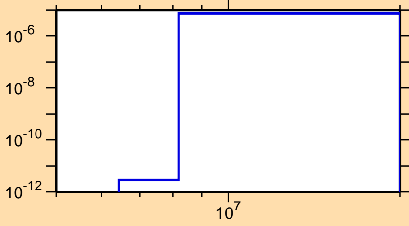
\sigma vs. E for ^{228}\text{Fr}(n,\alpha)
