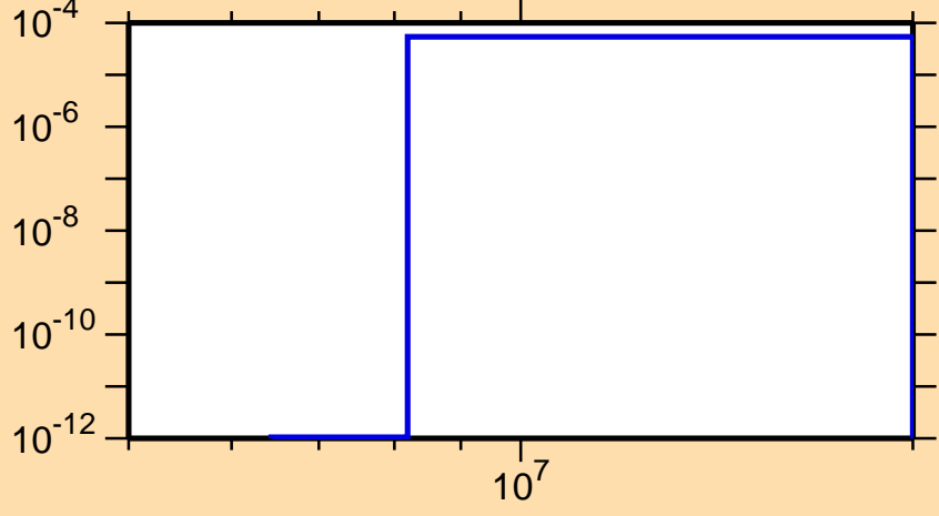
\sigma vs. E for ^{228}\text{Fr}(n,t)
