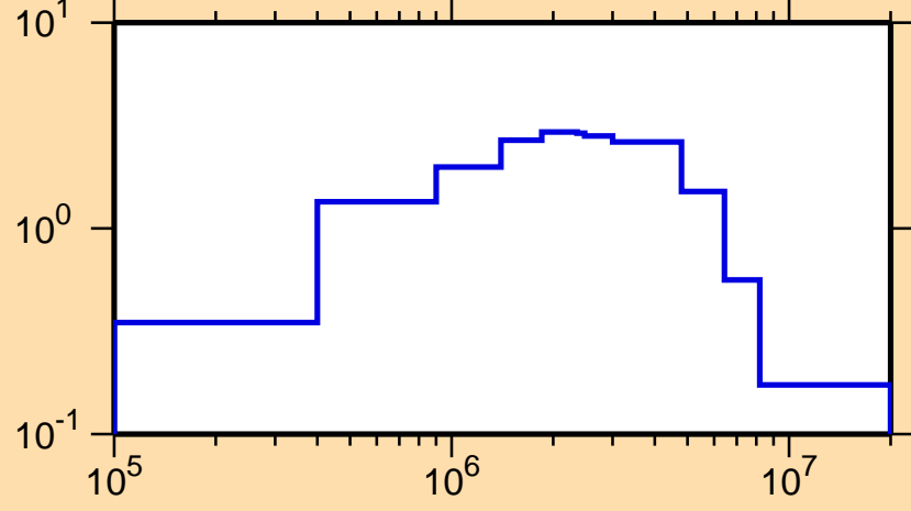
\sigma vs. E for ^{228}\text{Fr}(n,\text{inel.})
