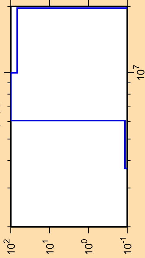
\Delta\sigma/\sigma vs. E for ^{229}\text{Fr}(n,p)
