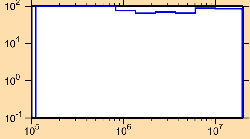
\Delta\sigma/\sigma vs. E for ^{229}\text{Fr}(n,\text{inel.})
