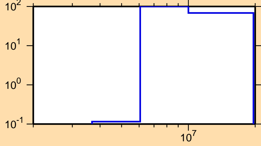
\Delta\sigma/\sigma vs. E for ^{229}\text{Fr}(n,p)
