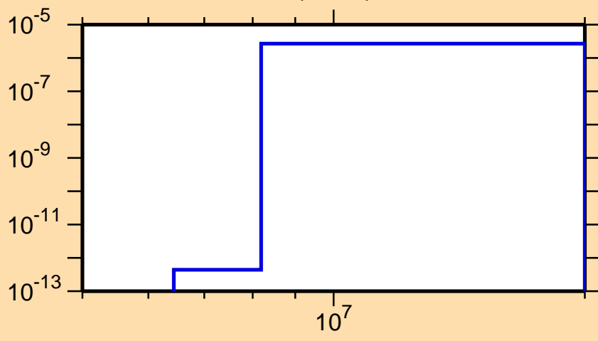
\sigma vs. E for ^{229}\text{Fr}(n,\alpha)
