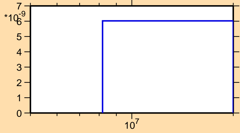
\sigma vs. E for ^{229}\text{Fr}(n,nd)
