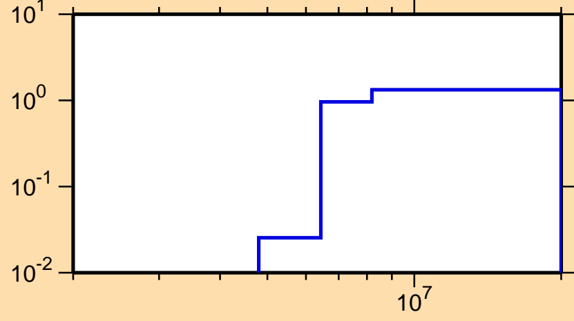
\sigma vs. E for ^{229}\text{Fr}(n,2n)
