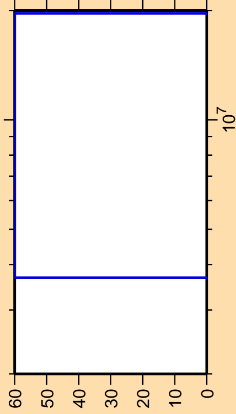
\Delta\sigma/\sigma vs. E for ^{230}\text{Fr}(n,n\text{cont.})
