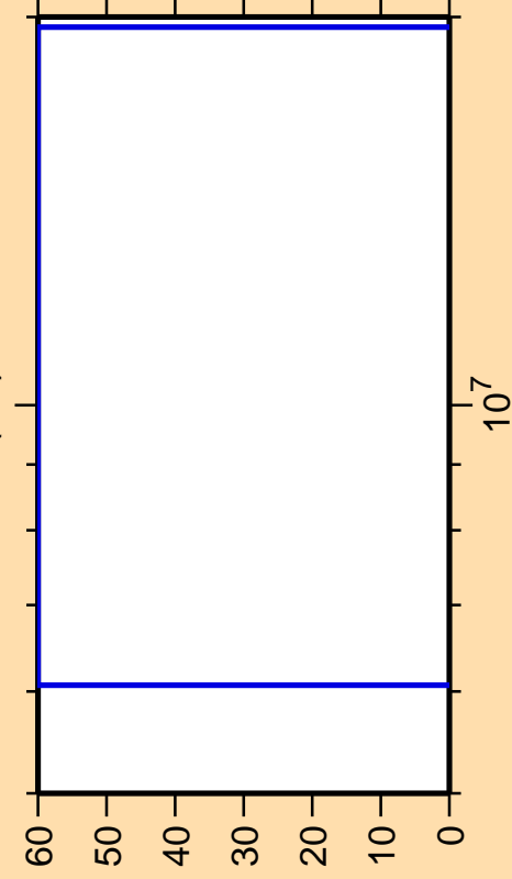
\Delta\sigma/\sigma vs. E for ^{230}\text{Fr}(n,t)
