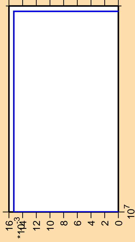
\Delta\sigma/\sigma vs. E for ^{230}\text{Fr} (mt 11)
