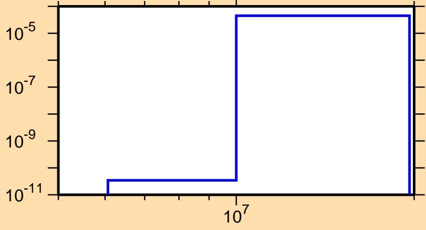
\sigma vs. E for ^{230}\text{Fr}(n,t)
