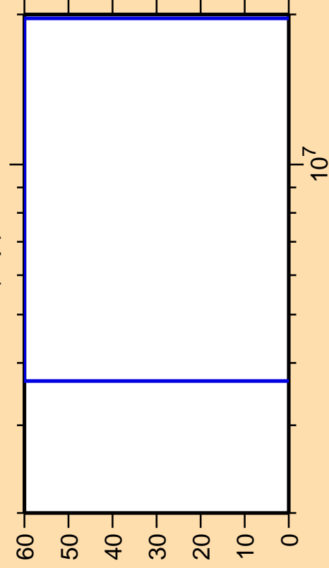
\Delta\sigma/\sigma vs. E for ^{230}\text{Fr}(n,p)
