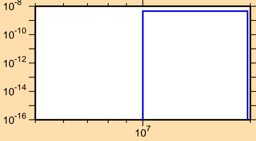
\sigma vs. E for ^{230}\text{Fr}(n,2n\alpha)
