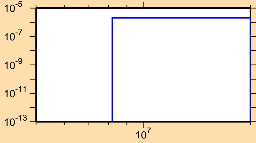
\sigma vs. E for ^{230}\text{Fr}(n,\alpha)
