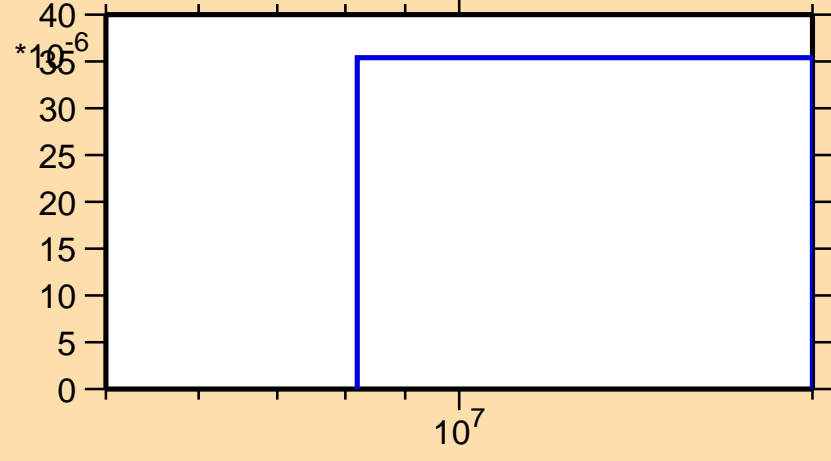
\sigma vs. E for ^{230}\text{Fr}(n,d)
