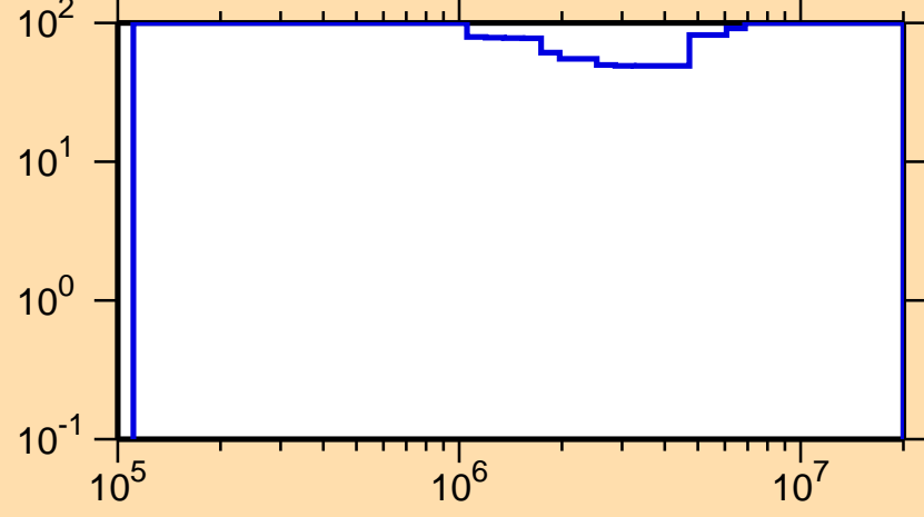
\Delta\sigma/\sigma vs. E for ^{231}\text{Fr}(n,n\text{cont.})
