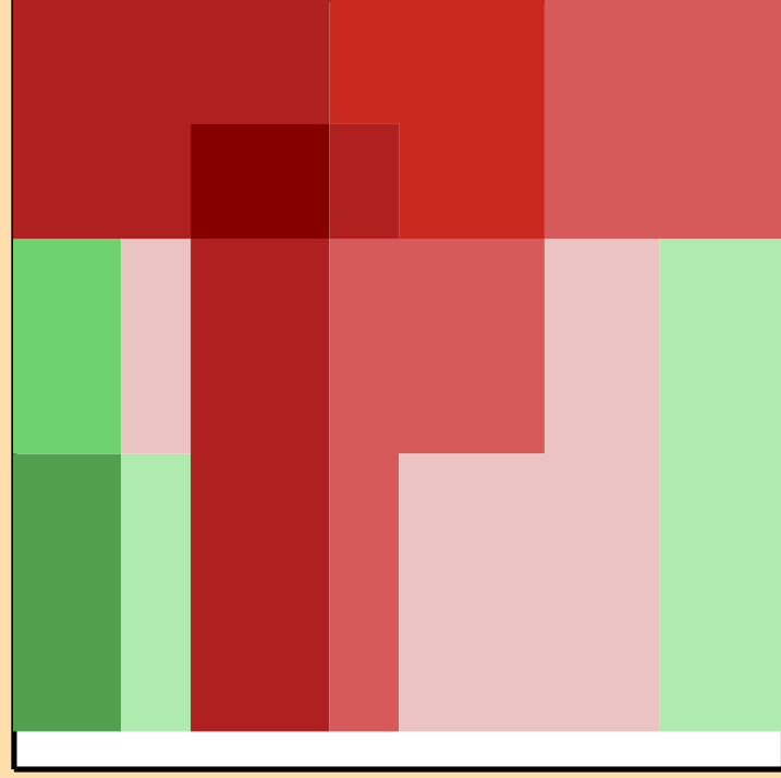
\Delta\sigma/\sigma vs. E for ^{231}\text{Fr}(n,\text{inel.})
