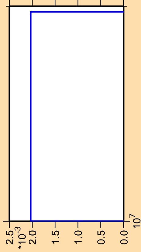
\Delta\sigma/\sigma vs. E for ^{231}\text{Fr}(\text{mt } 42)
