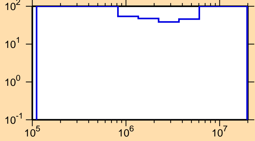
\Delta\sigma/\sigma vs. E for ^{231}\text{Fr}(n,\text{inel.})
