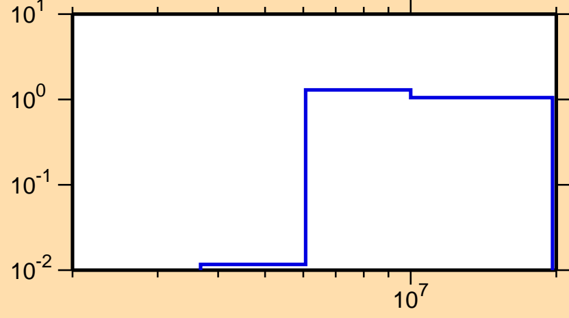
\sigma vs. E for ^{231}\text{Fr}(n,2n)
