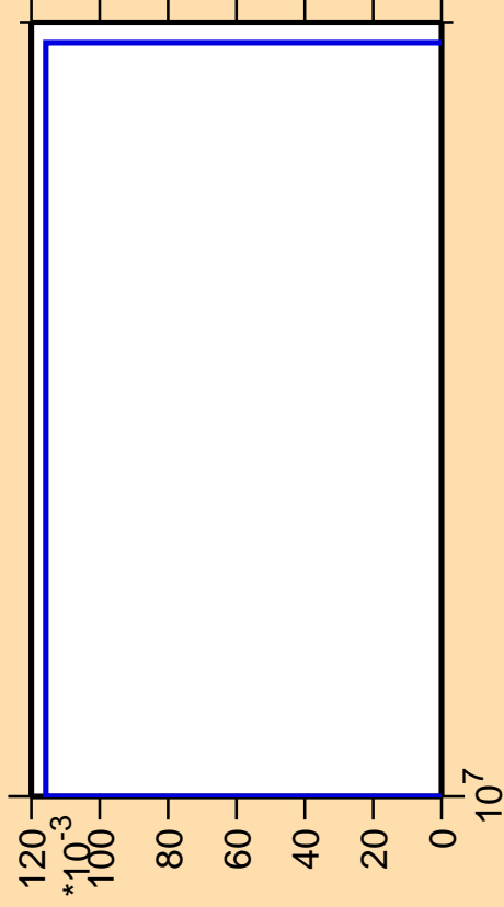
\Delta\sigma/\sigma vs. E for ^{231}\text{Fr}(n,3n\alpha)
