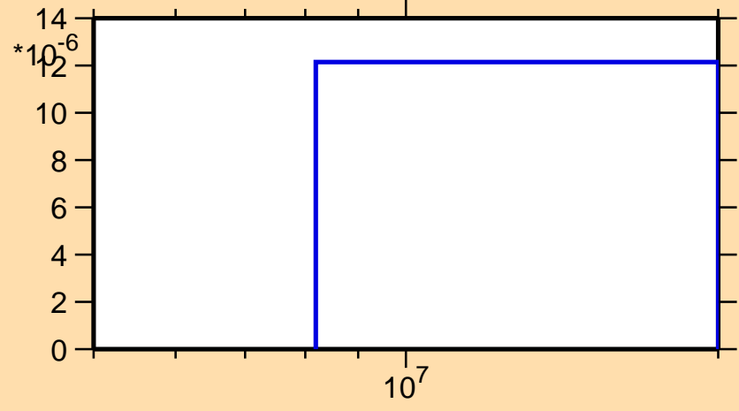
\sigma vs. E for ^{231}\text{Fr}(n,np)
