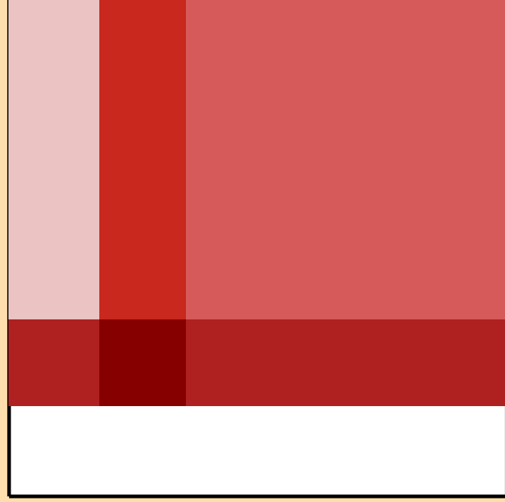
\Delta\sigma/\sigma vs. E for ^{231}\text{Fr}(n,2n)
