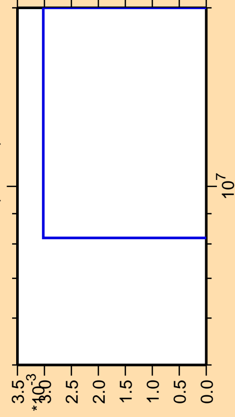
\Delta\sigma/\sigma vs. E for ^{231}\text{Fr}(\text{mt } 42)
