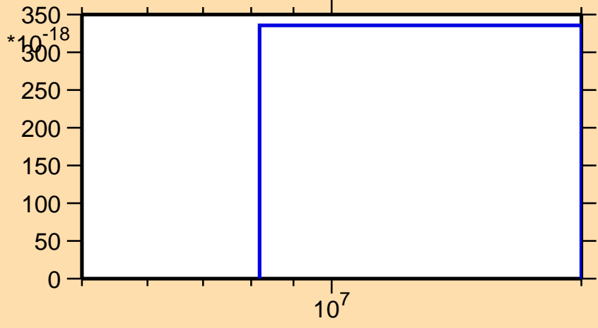
\sigma vs. E for ^{231}\text{Fr}(\text{mt } 42)
