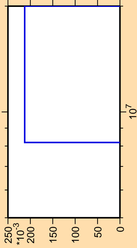
\Delta\sigma/\sigma vs. E for ^{231}\text{Fr}(\text{mt } 11)
