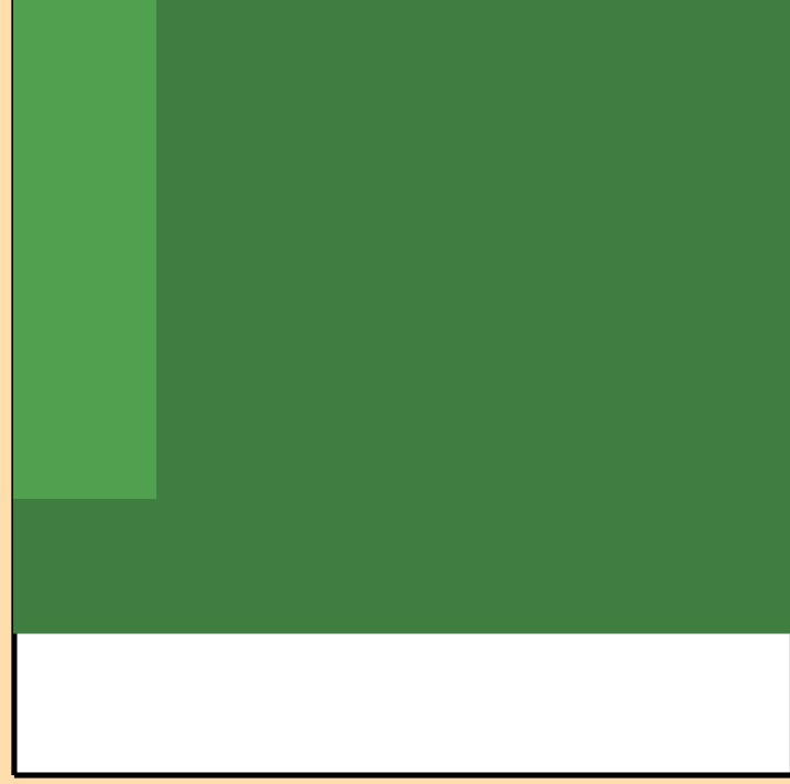
\Delta\sigma/\sigma vs. E for ^{231}\text{Fr}(n,el.)
