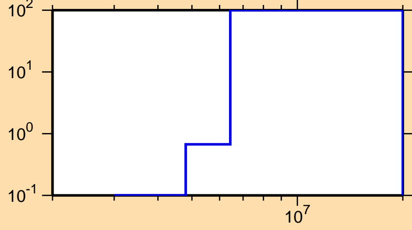
\Delta\sigma/\sigma vs. E for ^{231}\text{Fr}(n,f)
