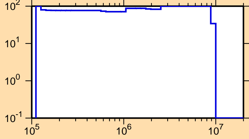
\Delta\sigma/\sigma vs. E for ^{232}\text{Fr}(n,n_1)
