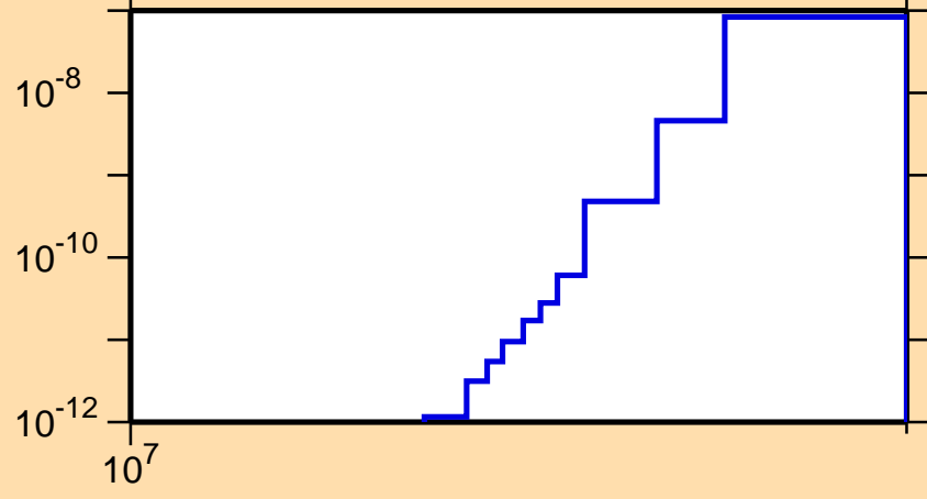
\sigma vs. E for ^{232}\text{Fr}(n,2n\alpha)
