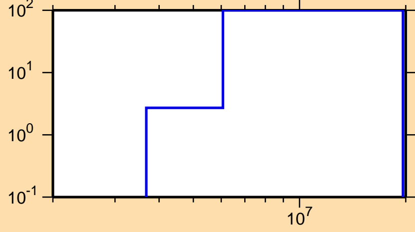
\Delta\sigma/\sigma vs. E for ^{232}\text{Fr}(n,f)
