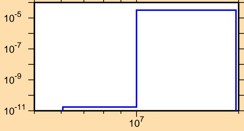
\sigma vs. E for ^{232}\text{Fr}(n,t)
