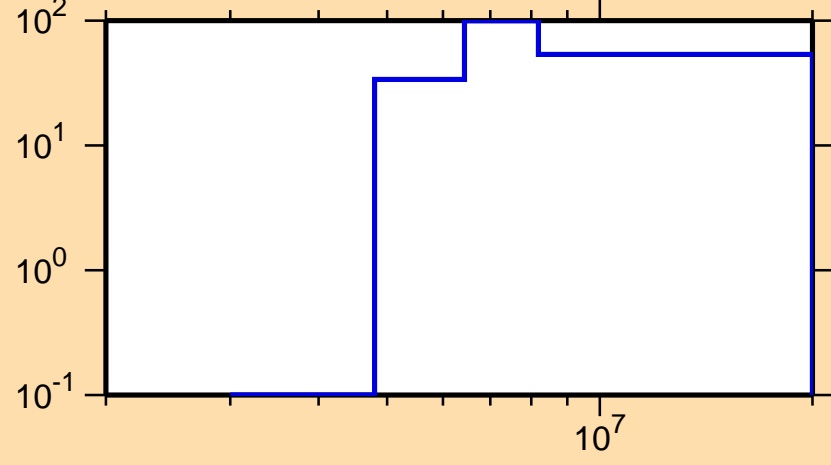
\Delta\sigma/\sigma vs. E for ^{232}\text{Fr}(n,p)
