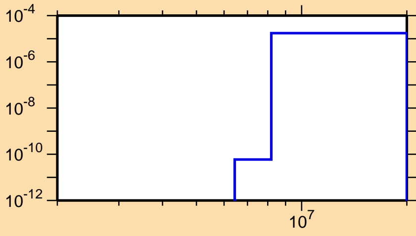
\sigma vs. E for ^{232}\text{Fr}(n,\alpha)
