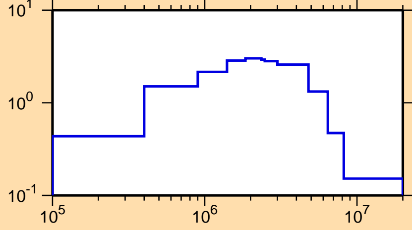
\sigma vs. E for ^{232}\text{Fr}(n,\text{inel.})
