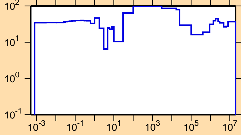
\Delta\sigma/\sigma vs. E for ^{232}\text{Fr}(n,\text{tot.})
