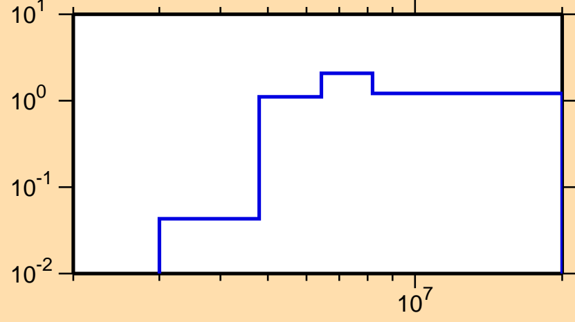
\sigma vs. E for ^{232}\text{Fr}(n,2n)
