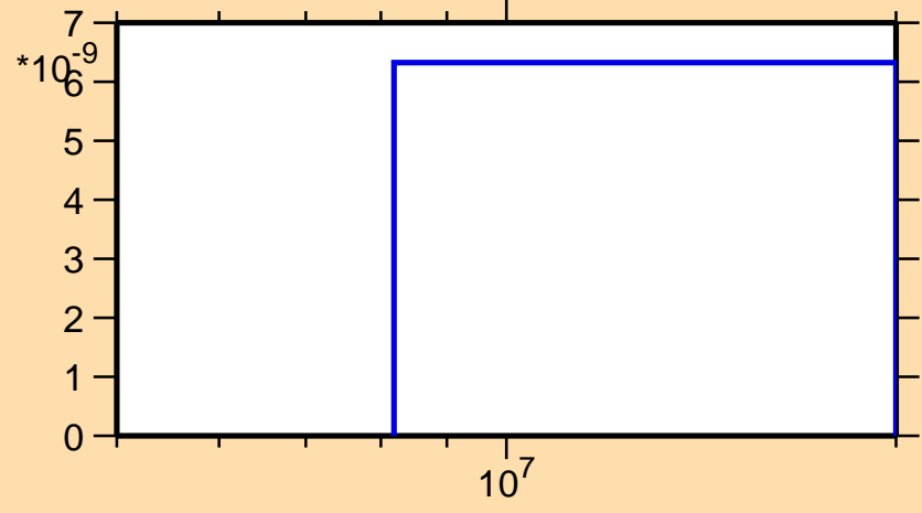
\sigma vs. E for ^{232}\text{Fr}(n,2np)
