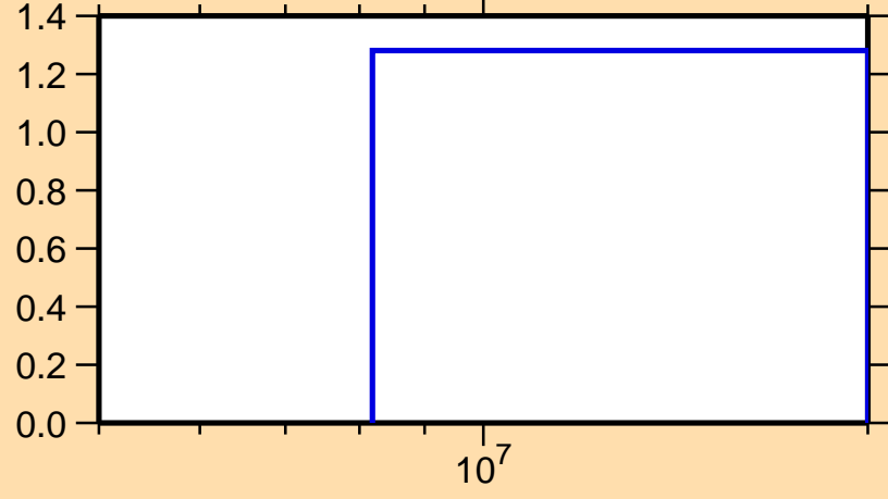
\sigma vs. E for ^{233}\text{Fr}(n,3n)
