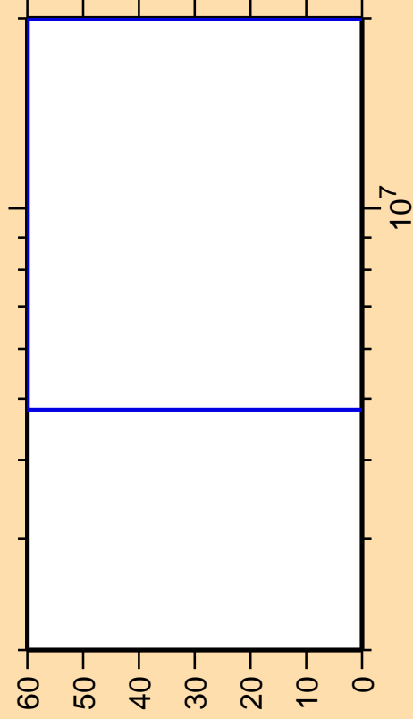
\Delta\sigma/\sigma vs. E for ^{233}\text{Fr}(n,\gamma)
