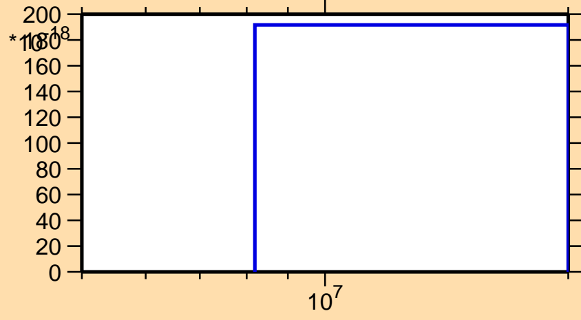
\sigma vs. E for ^{233}\text{Fr}(\text{mt } 42)
