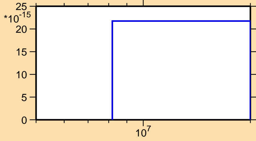
\sigma vs. E for ^{233}\text{Fr}(n,3n\alpha)
