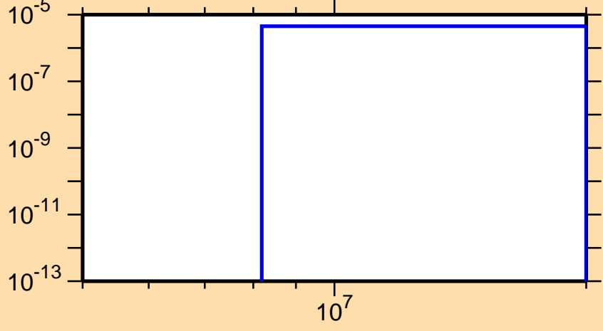
\sigma vs. E for ^{233}\text{Fr}(n,np)
