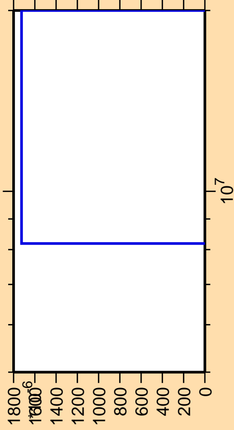
\Delta\sigma/\sigma vs. E for ^{233}\text{Fr}(\text{mt } 42)
