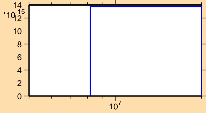
\sigma vs. E for ^{233}\text{Fr}(\text{mt 11})
