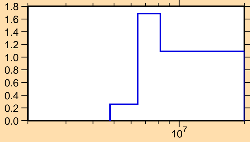
\sigma vs. E for ^{233}\text{Fr}(n,2n)
