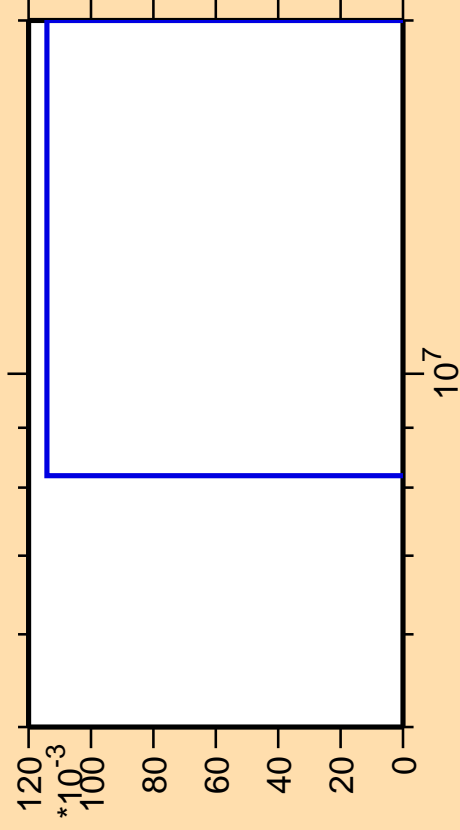
\Delta\sigma/\sigma vs. E for ^{233}\text{Fr}(\text{mt 11})
