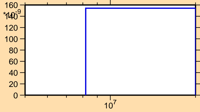
\sigma vs. E for ^{233}\text{Fr}(n,nt)
