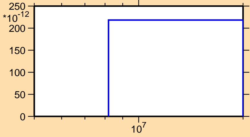
\sigma vs. E for ^{233}\text{Fr}(n,2np)
