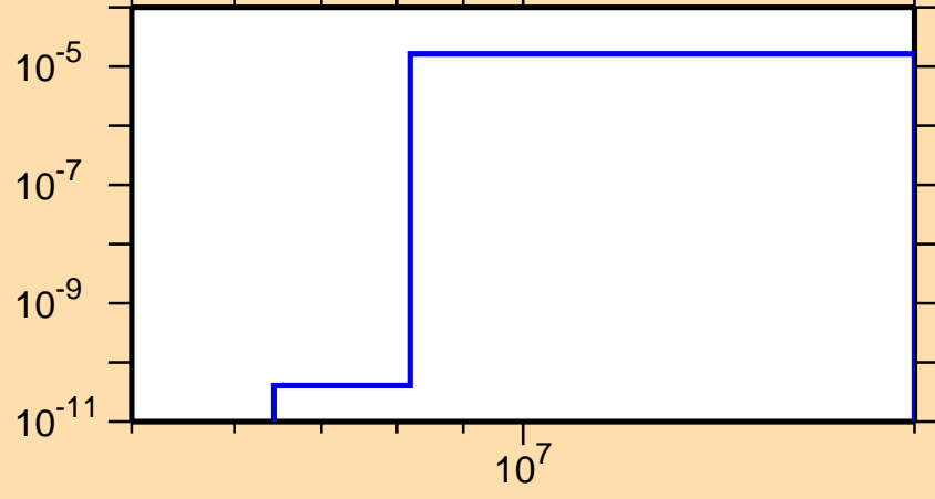
\sigma vs. E for ^{233}\text{Fr}(n,\alpha)
