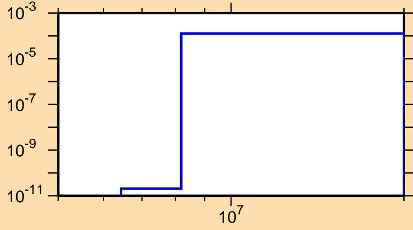
\sigma vs. E for ^{233}\text{Fr}(n,p)
