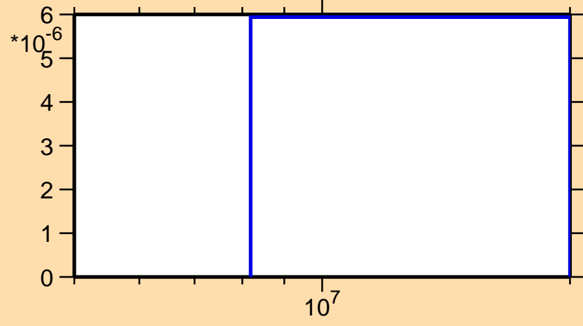
\sigma vs. E for ^{233}\text{Fr}(n,t)
