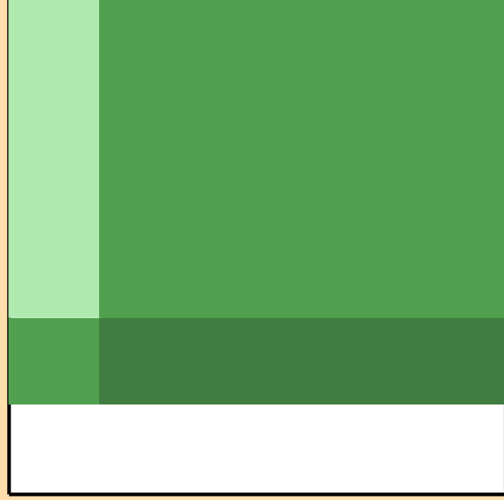
\Delta\sigma/\sigma vs. E for ^{233}\text{Fr}(n,\text{el.})
