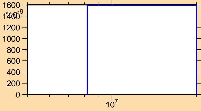
\sigma vs. E for ^{233}\text{Fr}(n,\alpha)
