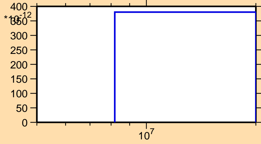
\sigma vs. E for ^{233}\text{Fr}(n,2n\alpha)
