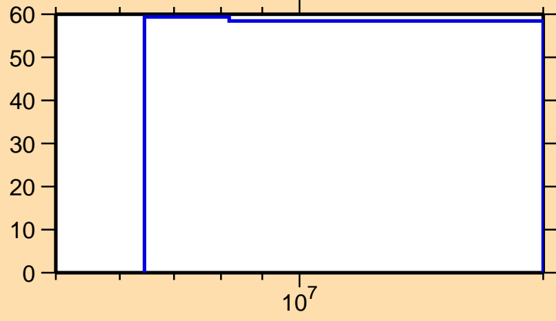
\Delta\sigma/\sigma vs. E for ^{233}\text{Fr}(n,\text{nonel.})
