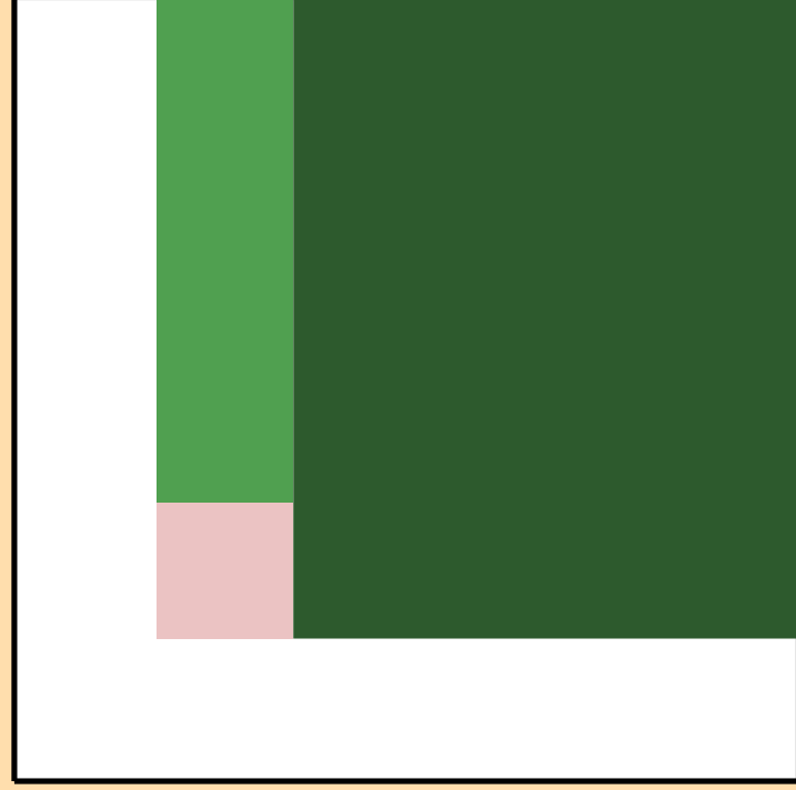
\Delta\sigma/\sigma vs. E for ^{233}\text{Fr}(n,p)
