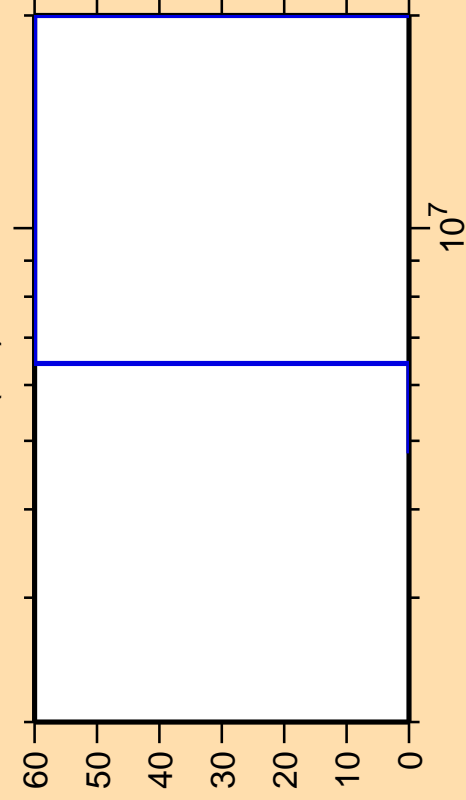
\Delta\sigma/\sigma vs. E for ^{233}\text{Fr}(n,f)
