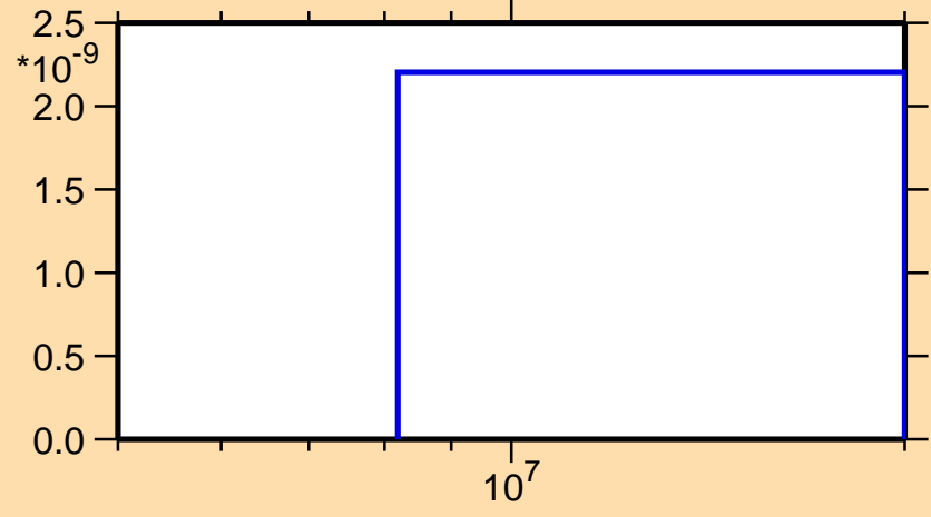
\sigma vs. E for ^{233}\text{Fr}(n,\text{nd})
