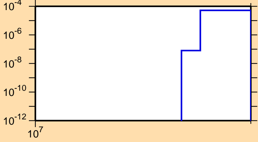
\sigma vs. E for ^{63}\text{Ga}(n,2np)
