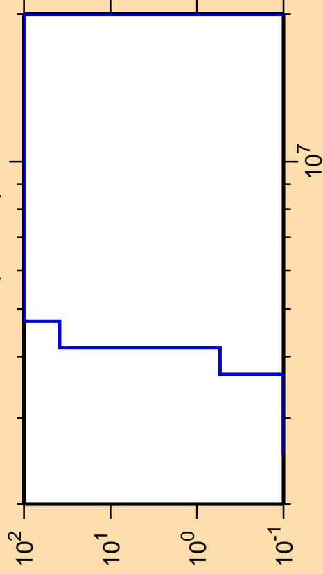
\Delta\sigma/\sigma vs. E for ^{63}\text{Ga}(n,\text{He}3)
