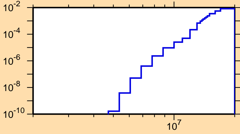
\sigma vs. E for ^{63}\text{Ga}(n,\text{He}3)
