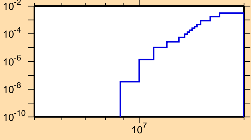
\sigma vs. E for ^{63}\text{Ga}(n,t)
