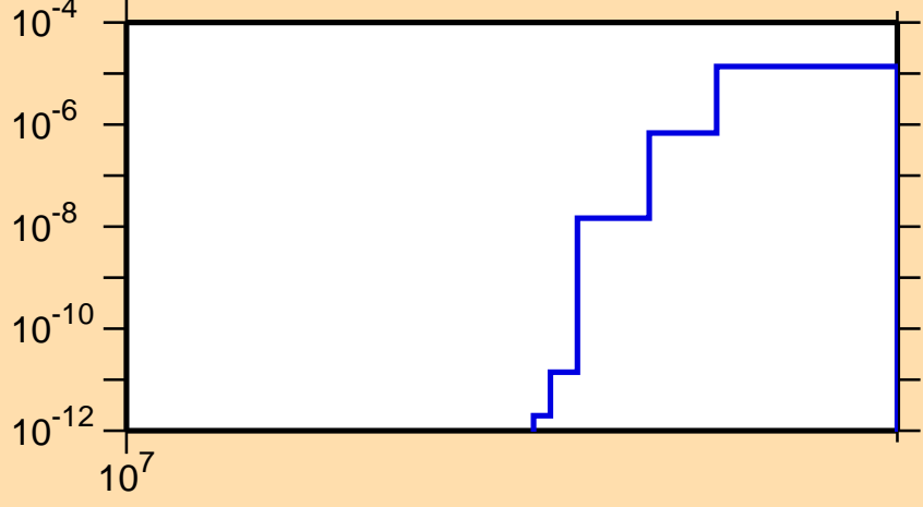
\sigma vs. E for ^{63}\text{Ga}(n,\text{nd})
