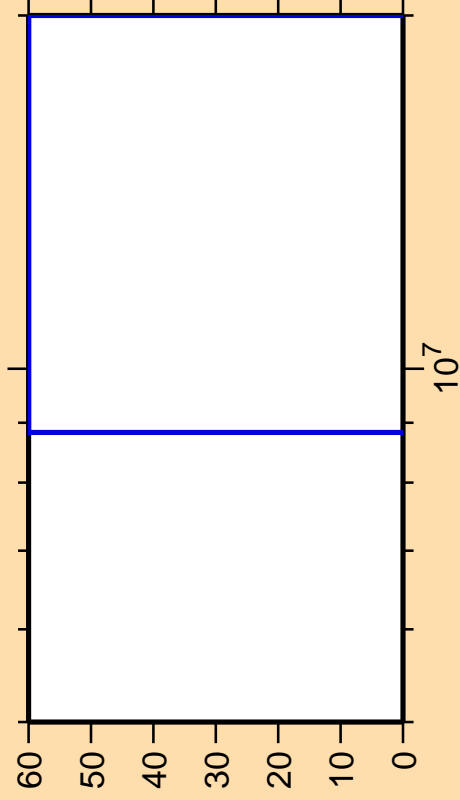
\Delta\sigma/\sigma vs. E for ^{63}\text{Ga}(n,pd)
