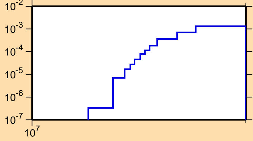
\sigma vs. E for ^{63}\text{Ga}(n,2n)
