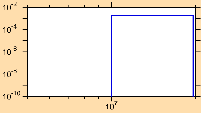
\sigma vs. E for ^{63}\text{Ga}(n,pd)
