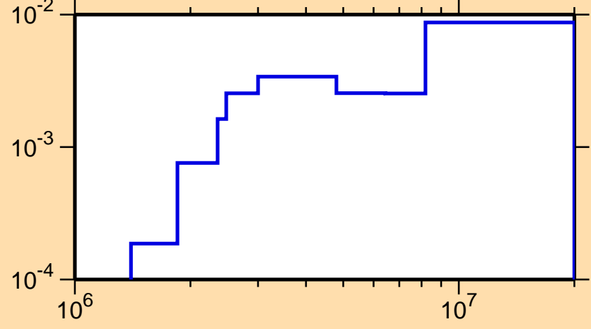
\sigma vs. E for ^{63}\text{Ga}(n,n\text{cont.})
