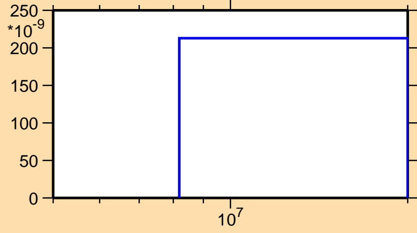
\sigma vs. E for ^{63}\text{Ga}(n,\text{pt})
