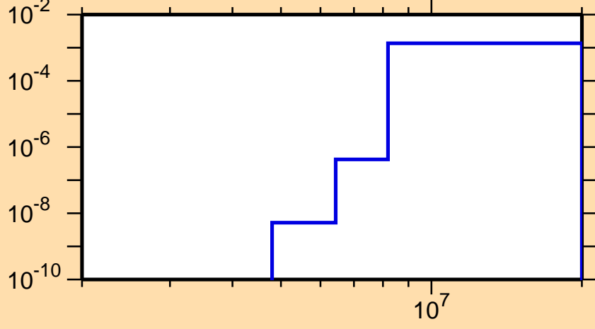
\sigma vs. E for ^{63}\text{Ga}(n,\text{He}3)
