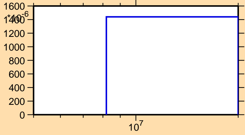
\sigma vs. E for ^{63}\text{Ga}(n,\text{pd})
