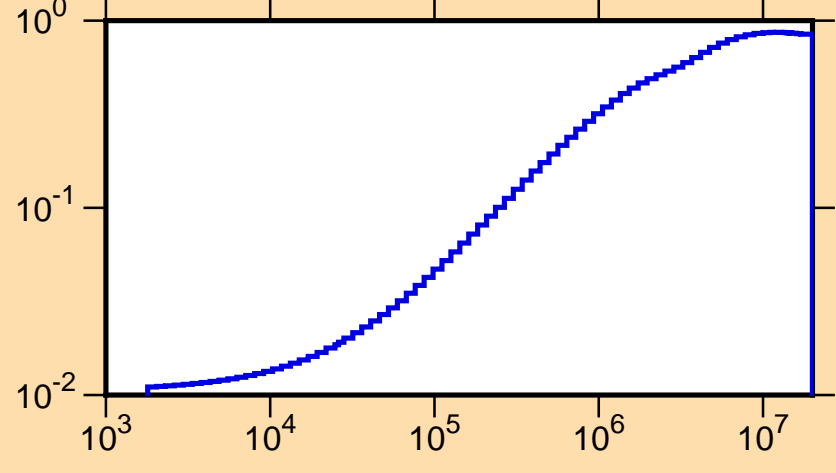
\mu vs. E for ^{64}\text{Ga}(\text{mt251})
