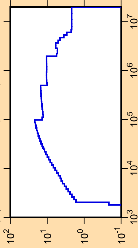
\Delta\mu/\mu vs. E for ^{64}\text{Ga}(\text{mt251})
