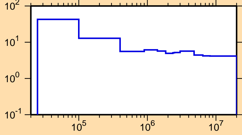
\Delta\sigma/\sigma vs. E for ^{64}\text{Ga}(n,\text{nonel.})
