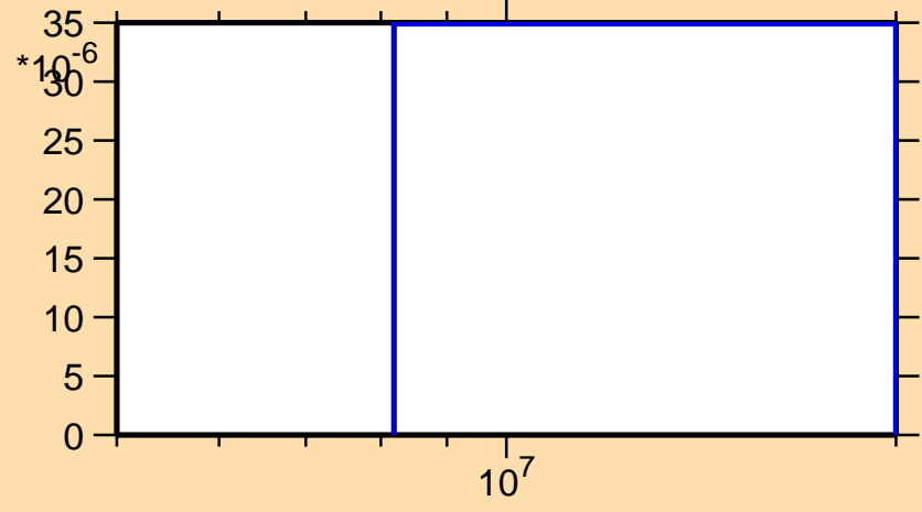
\sigma vs. E for ^{64}\text{Ga}(n,\text{nd})
