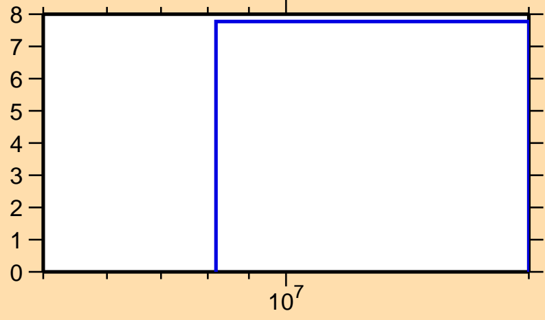
\Delta\sigma/\sigma vs. E for ^{64}\text{Ga}(n,\text{el.})
