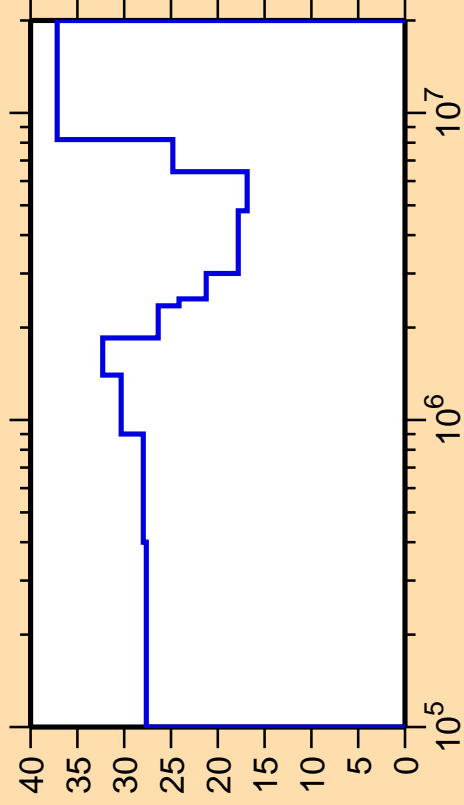
\Delta\sigma/\sigma vs. E for ^{64}\text{Ga}(n,n_3)
