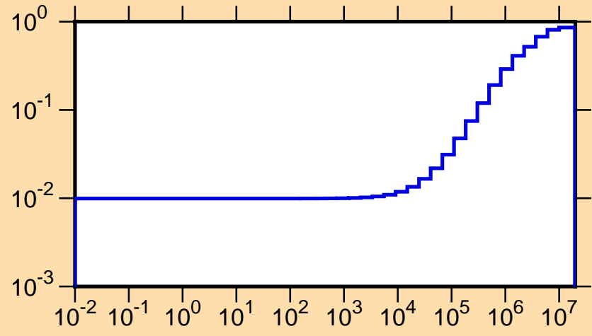
\mu vs. E for ^{68}\text{Ga}(\text{mt251})
