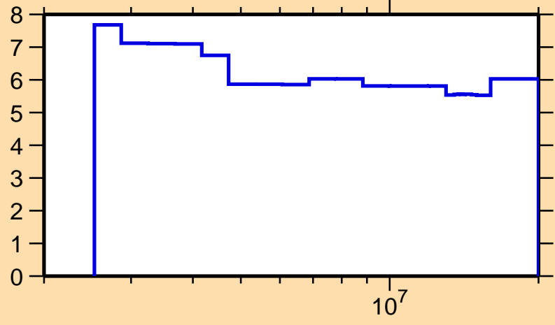
\Delta\sigma/\sigma vs. E for ^{69}\text{Ga}(n,n\text{onl.})
