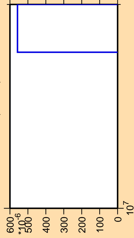
\Delta\sigma/\sigma vs. E for ^{69}\text{Ga} (mt 34)
