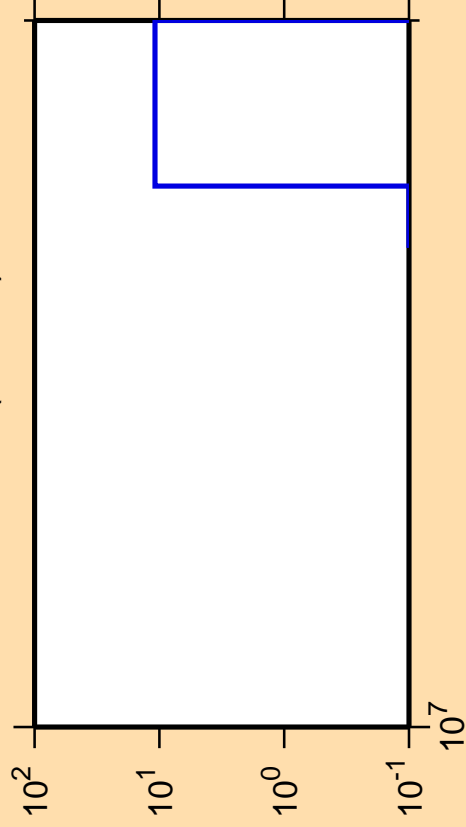
\Delta\sigma/\sigma vs. E for ^{70}\text{Ga}(\text{mt117})
