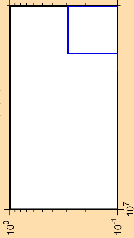
\Delta\sigma/\sigma vs. E for ^{70}\text{Ga}(n,pd)
