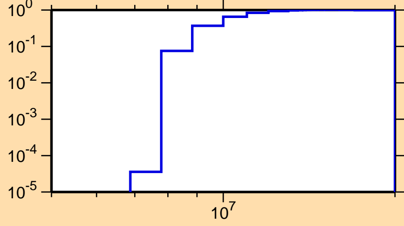
\sigma vs. E for ^{70}\text{Ga}(n,2n)
