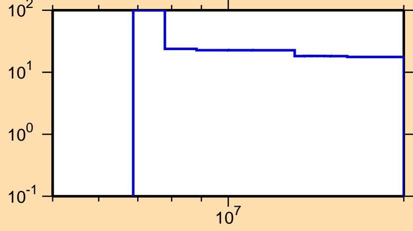
\Delta\sigma/\sigma vs. E for ^{70}\text{Ga}(n,2n)
