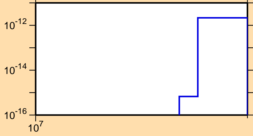
\sigma vs. E for ^{70}\text{Ga}(\text{mt117})
