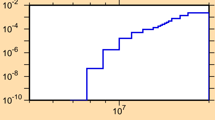
\sigma vs. E for ^{70}\text{Ga}(n,t)
