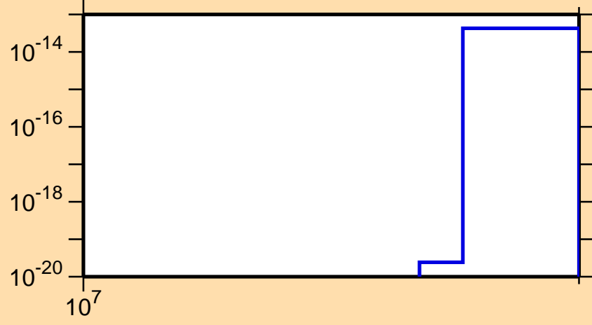
\sigma vs. E for ^{70}\text{Ga}(n,pd)
