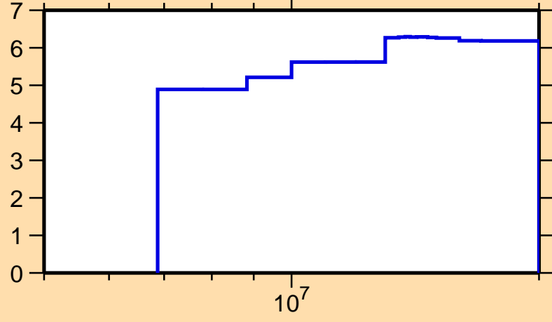
\Delta\sigma/\sigma vs. E for ^{70}\text{Ga}(n,\text{tot.})
