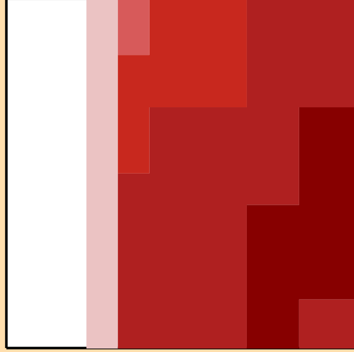
\Delta\sigma/\sigma vs. E for ^{70}\text{Ga}(n,2n)
