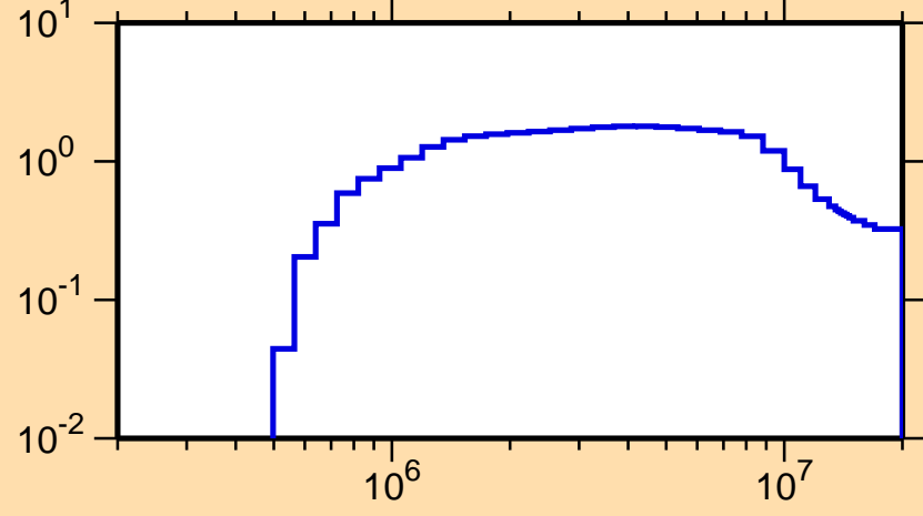
\sigma vs. E for ^{70}\text{Ga}(n,\text{inel.})
