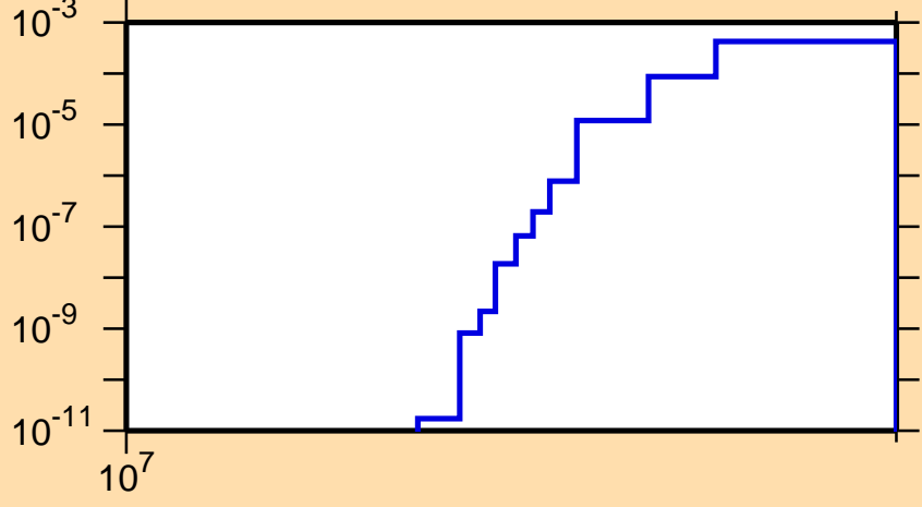
\sigma vs. E for ^{70}\text{Ga}(n,\text{nd})
