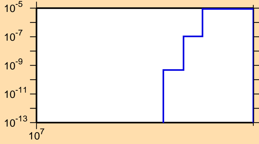
\sigma vs. E for ^{70}\text{Ga}(n,2n\alpha)
