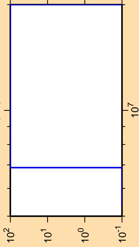
\Delta\sigma/\sigma vs. E for ^{70}\text{Ga}(n,t)
