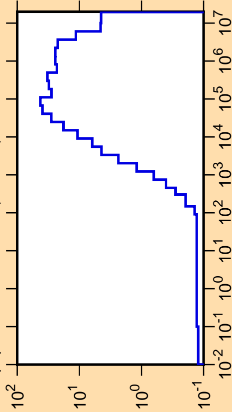
\Delta\mu/\mu vs. E for ^{70}\text{Ga}(\text{mt251})
