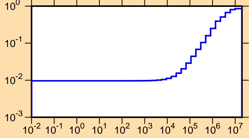
\mu vs. E for ^{70}\text{Ga}(\text{mt251})
