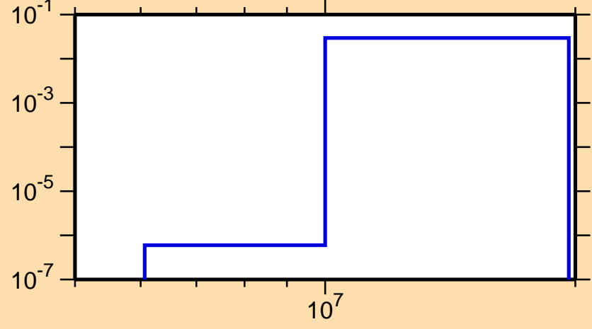
\sigma vs. E for ^{70}\text{Ga}(n,np)
