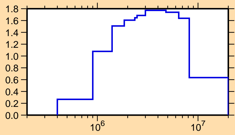
\sigma vs. E for ^{70}\text{Ga}(n,\text{inel.})
