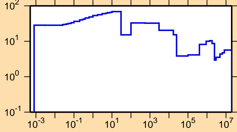
\Delta\sigma/\sigma vs. E for ^{70}\text{Ga}(n,\text{tot.})
