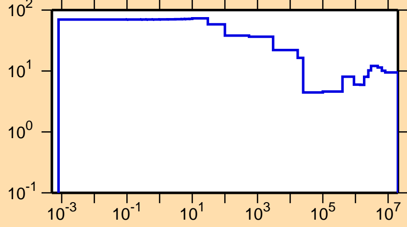
\Delta\sigma/\sigma vs. E for ^{70}\text{Ga}(n,\text{el.})
