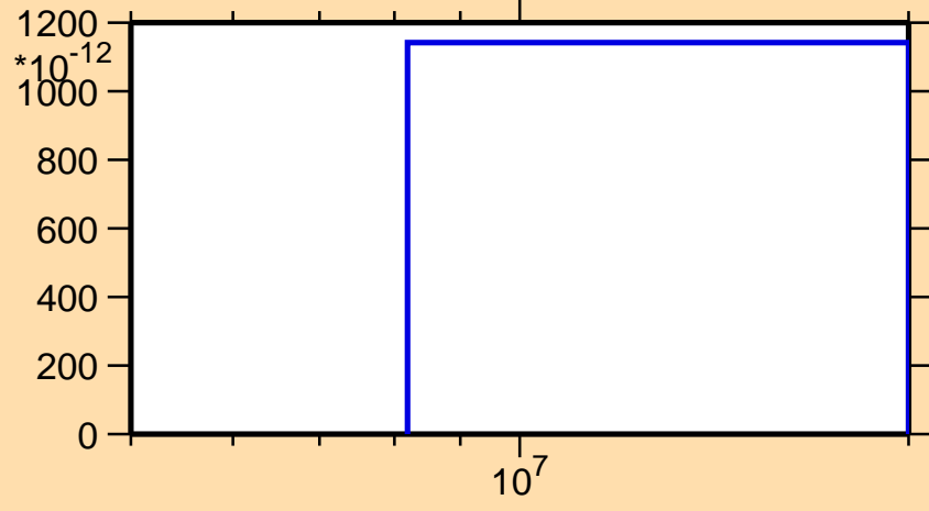
\sigma vs. E for ^{70}\text{Ga}(n,nt)
