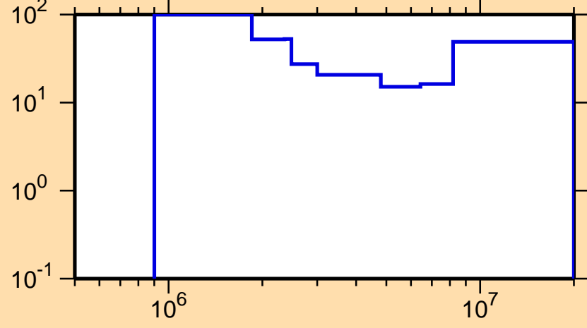
\Delta\sigma/\sigma vs. E for ^{70}\text{Ga}(n,n\text{cont.})
