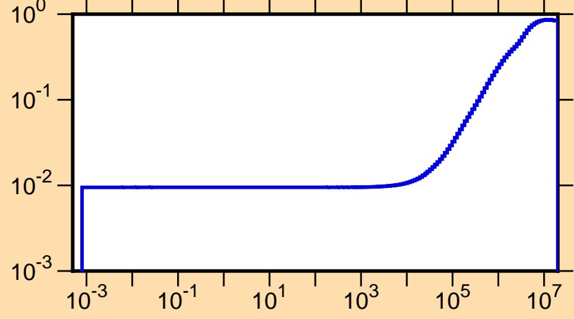
\mu vs. E for ^{71}\text{Ga}(\text{mt251})
