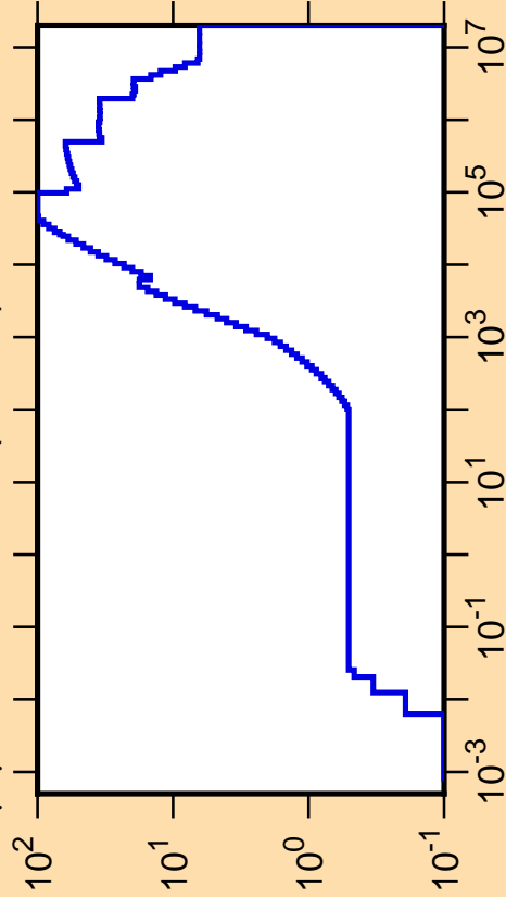
\Delta\mu/\mu vs. E for ^{71}\text{Ga}(\text{mt251})
