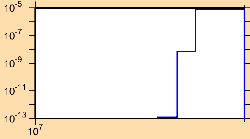
\sigma vs. E for ^{71}\text{Ga}(n,\text{nd})
