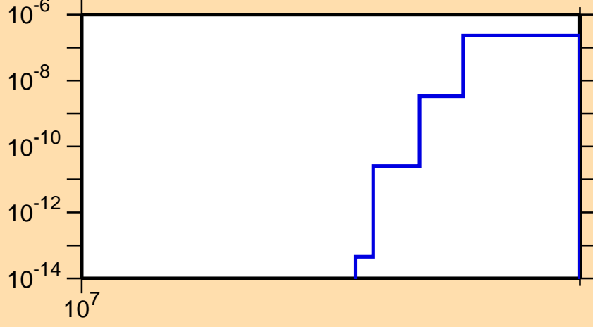
\sigma vs. E for ^{71}\text{Ga}(n,\text{He}3)
