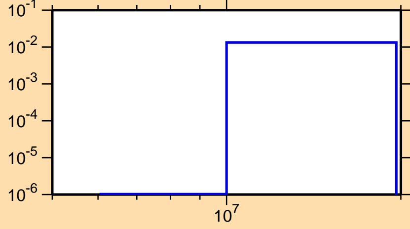
\sigma vs. E for ^{71}\text{Ga}(n,np)
