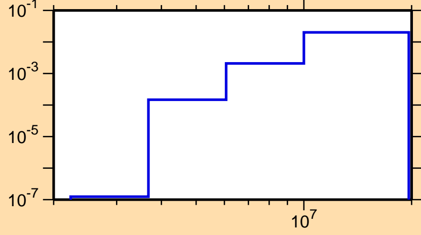
\sigma vs. E for ^{71}\text{Ga}(n,p)
