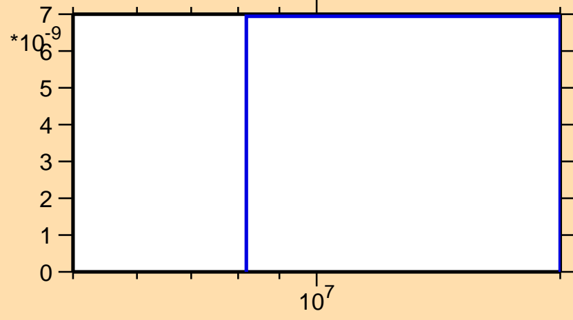
\sigma vs. E for ^{71}\text{Ga}(n,\text{nt})
