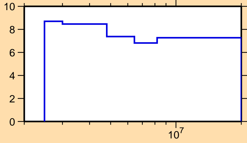
\Delta\sigma/\sigma vs. E for ^{71}\text{Ga}(n,n\text{onel.})
