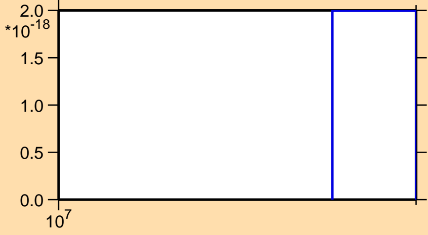
\sigma vs. E for ^{72}\text{Ga}(n,pd)
