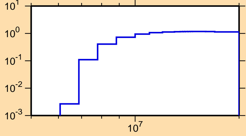
\sigma vs. E for ^{72}\text{Ga}(n,2n)
