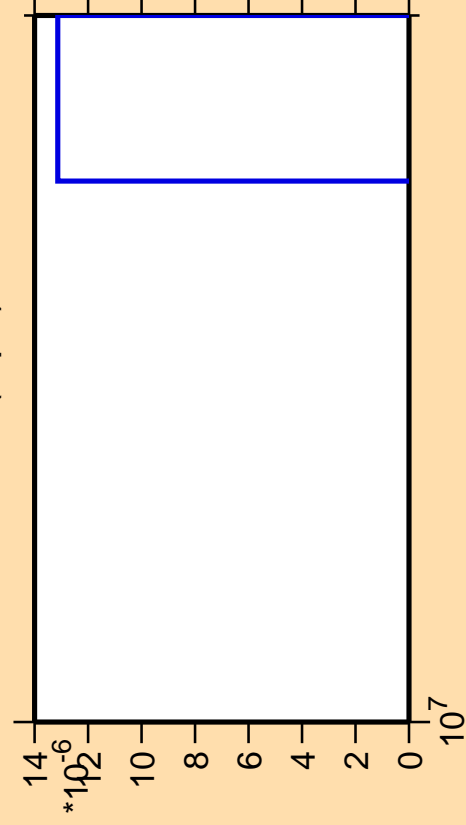
\Delta\sigma/\sigma vs. E for ^{72}\text{Ga}(n,pd)
