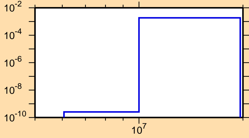
\sigma vs. E for ^{72}\text{Ga}(n,n\alpha)
