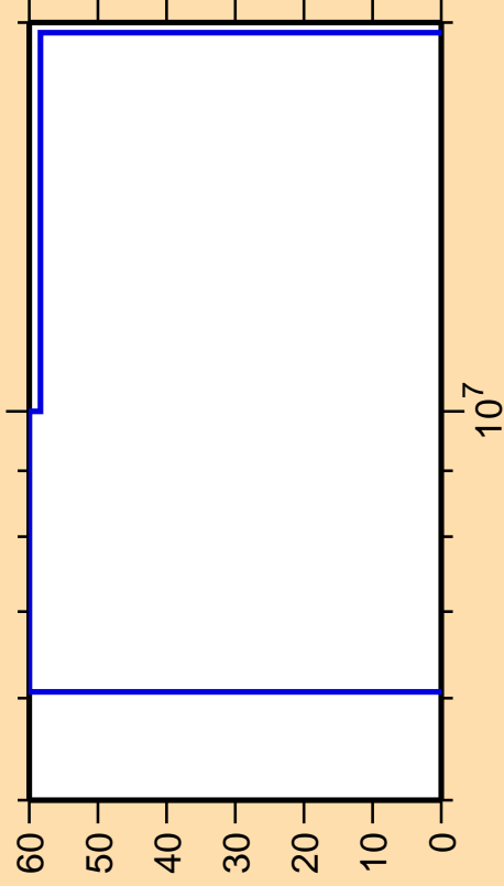
\Delta\sigma/\sigma vs. E for ^{72}\text{Ga}(n,n\alpha)
