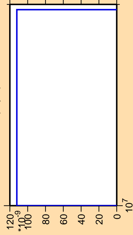
\Delta\sigma/\sigma vs. E for ^{72}\text{Ga}(n,\text{pd})
