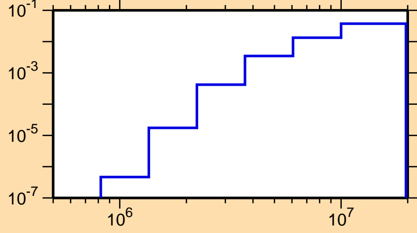
\sigma vs. E for ^{72}\text{Ga}(n,p)
