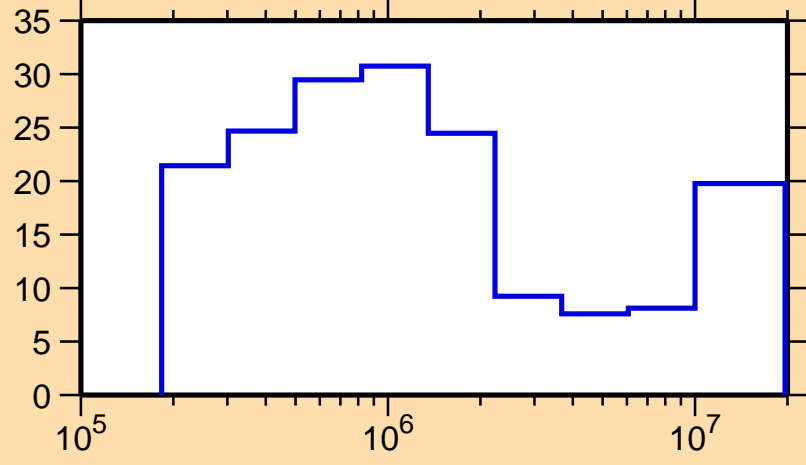
\Delta\sigma/\sigma vs. E for ^{72}\text{Ga}(n,el.)
