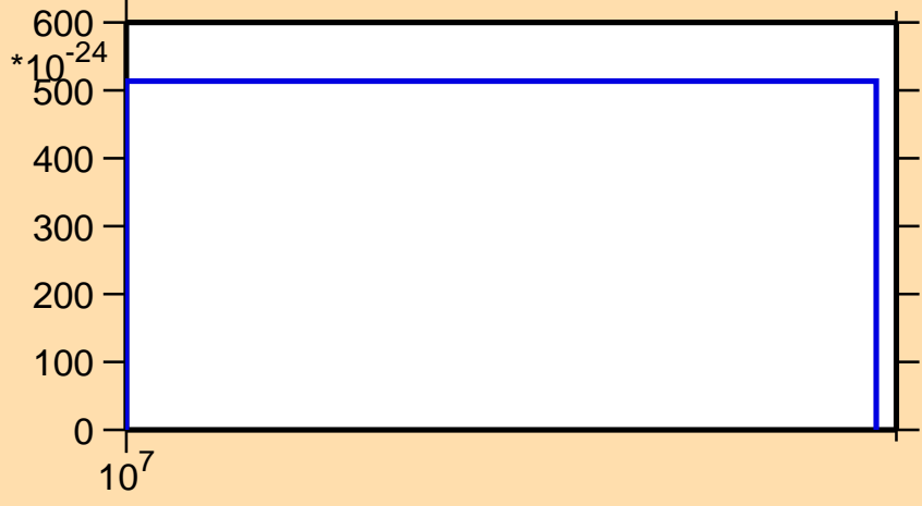
\sigma vs. E for ^{72}\text{Ga} (mt 34)
