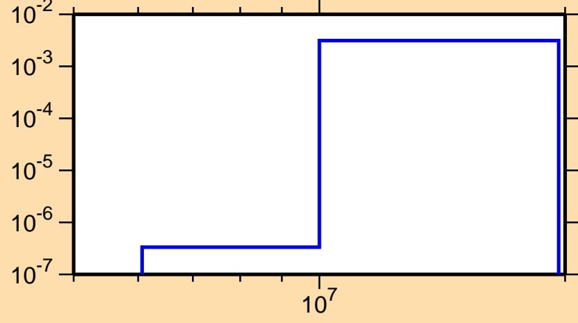
\sigma vs. E for ^{72}\text{Ga}(n,d)
