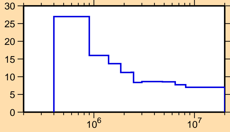
\Delta\sigma/\sigma vs. E for ^{72}\text{Ga}(n,n\text{onel.})
