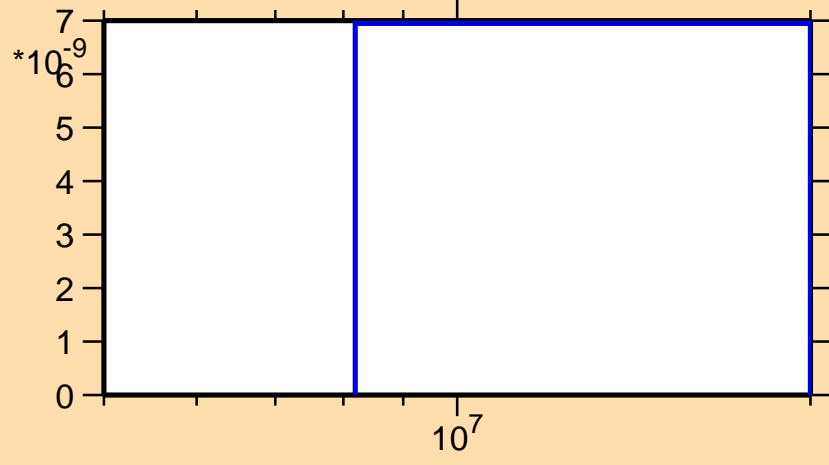
\sigma vs. E for ^{72}\text{Ga}(n,nt)
