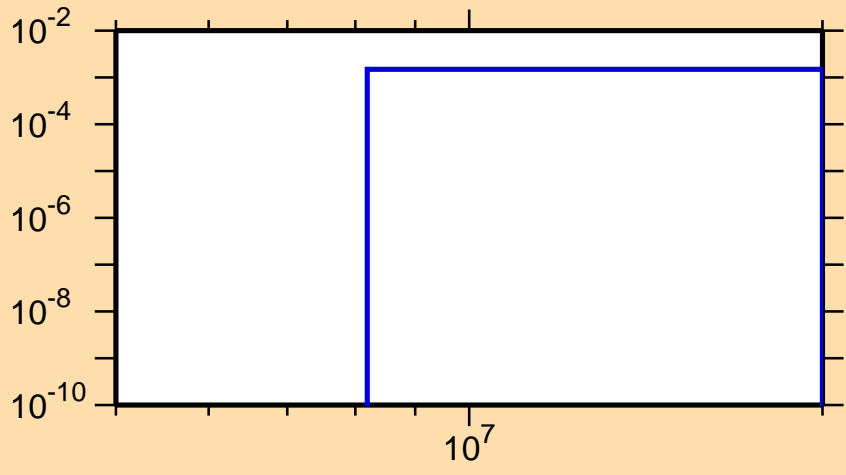
\sigma vs. E for ^{72}\text{Ga}(n,n\alpha)
