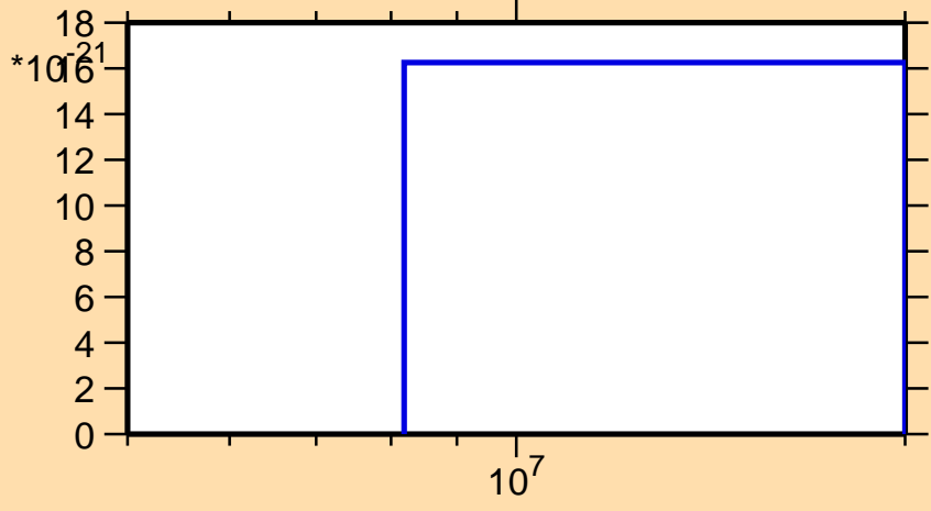
\sigma vs. E for ^{72}\text{Ga}(n,\text{pd})
