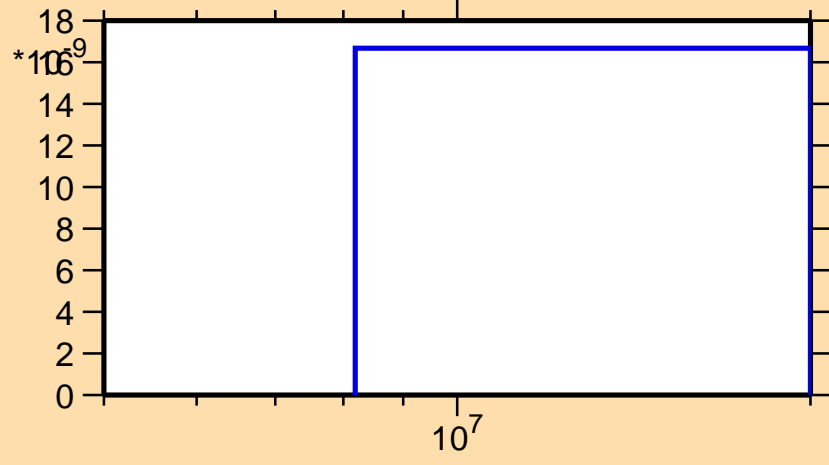
\sigma vs. E for ^{72}\text{Ga}(n,2n\alpha)
