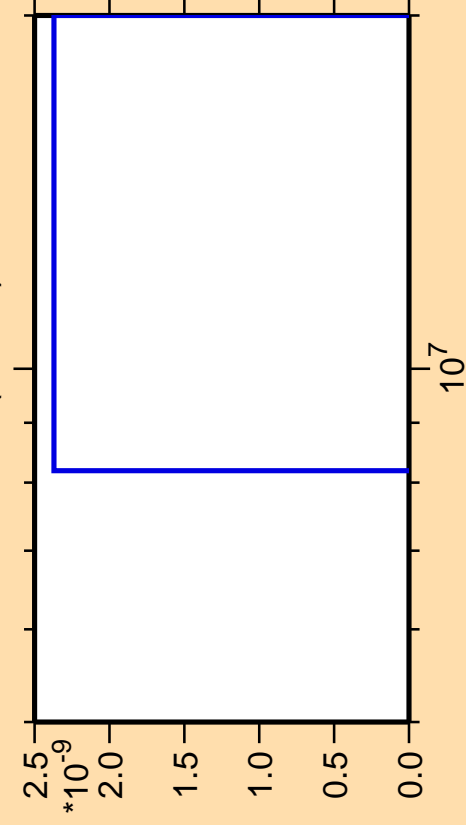
\Delta\sigma/\sigma vs. E for ^{72}\text{Ga} (mt 34)
