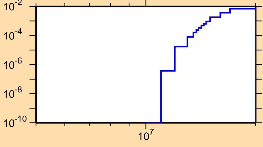
\sigma vs. E for ^{74}\text{Ga}(n,np)
