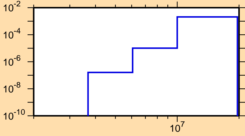
\sigma vs. E for ^{74}\text{Ga}(n,\alpha)
