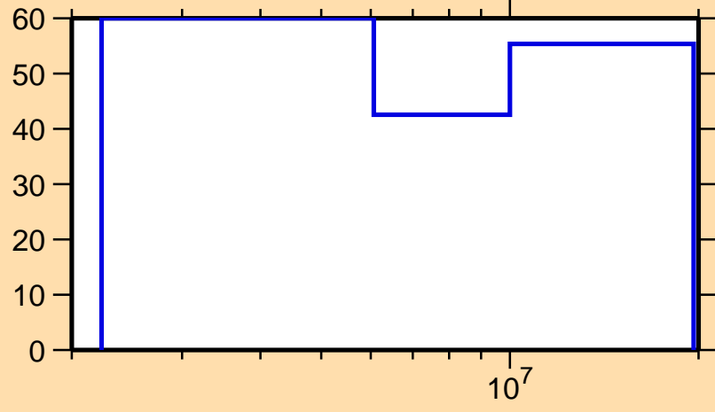
\Delta\sigma/\sigma vs. E for ^{74}\text{Ga}(n,p)
