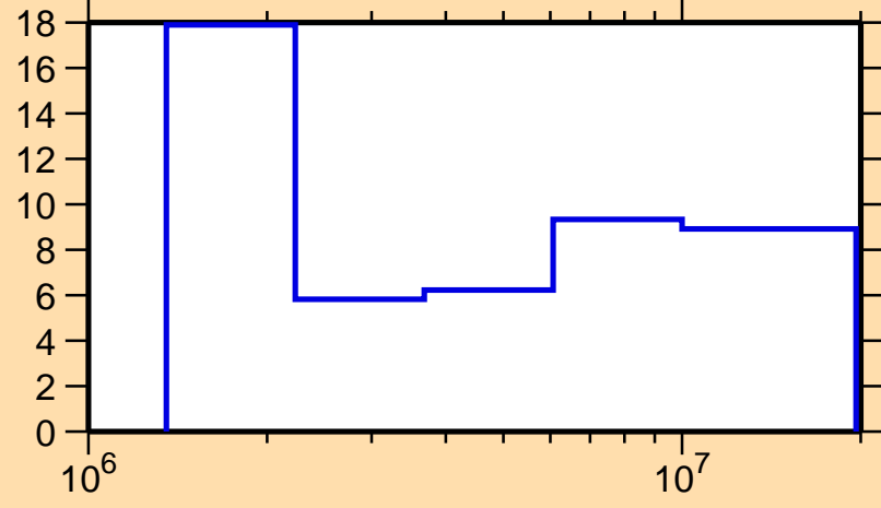
\Delta\sigma/\sigma vs. E for ^{74}\text{Ga}(n,n\text{inel.})
