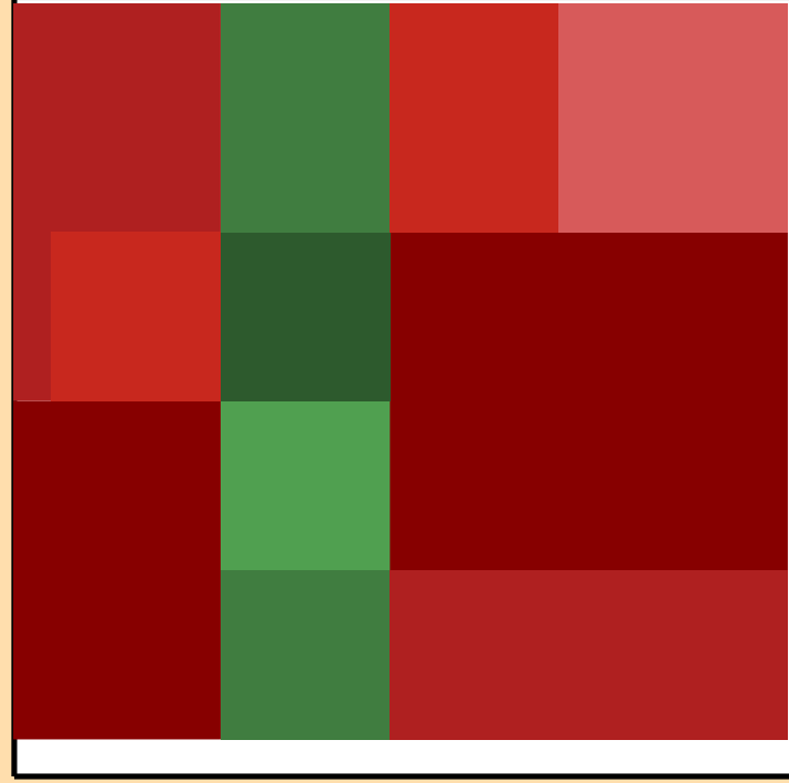
\Delta\sigma/\sigma vs. E for ^{74}\text{Ga}(n,n\text{cont.})
