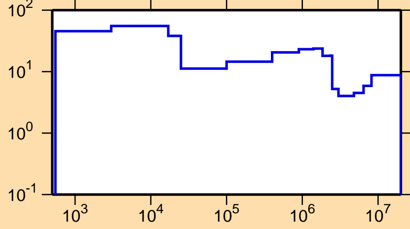
\Delta\sigma/\sigma vs. E for ^{74}\text{Ga}(n,\text{tot.})
