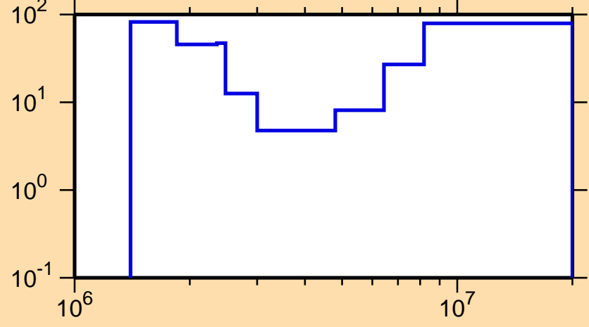
\Delta\sigma/\sigma vs. E for ^{74}\text{Ga}(n,n\text{cont.})
