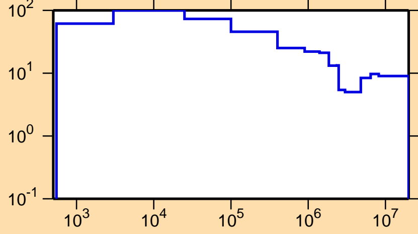
\Delta\sigma/\sigma vs. E for ^{74}\text{Ga}(n,\text{nonel.})
