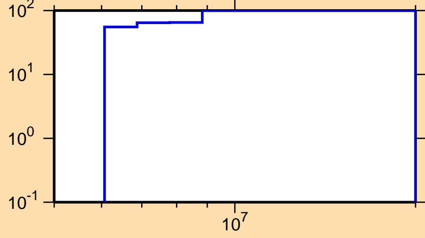
\Delta\sigma/\sigma vs. E for ^{77}\text{Ga}(n,n_1)
