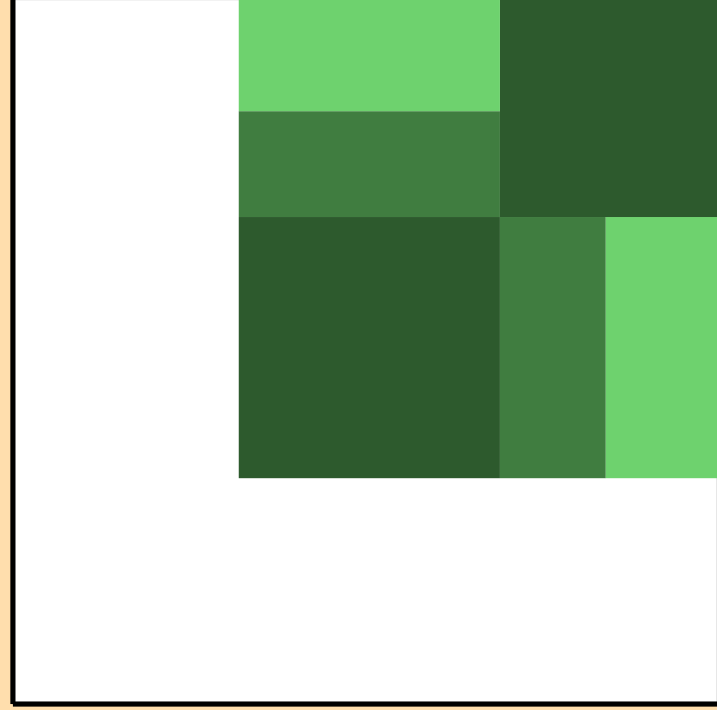
\sigma vs. E for ^{77}\text{Ga}(n,2n)
