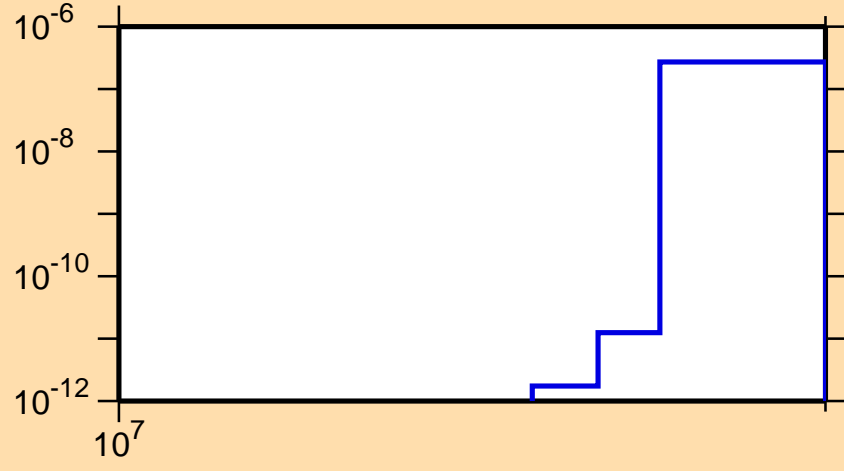
\sigma vs. E for ^{77}\text{Ga}(n,nt)
