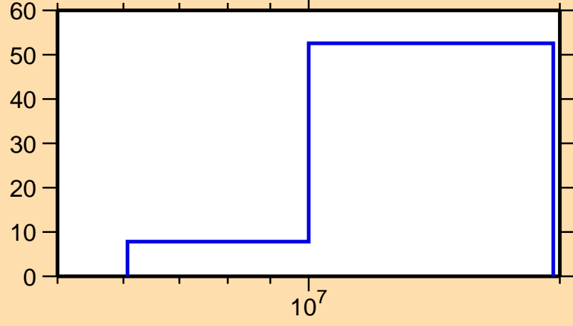
\Delta\sigma/\sigma vs. E for ^{77}\text{Ga}(n,el.)
