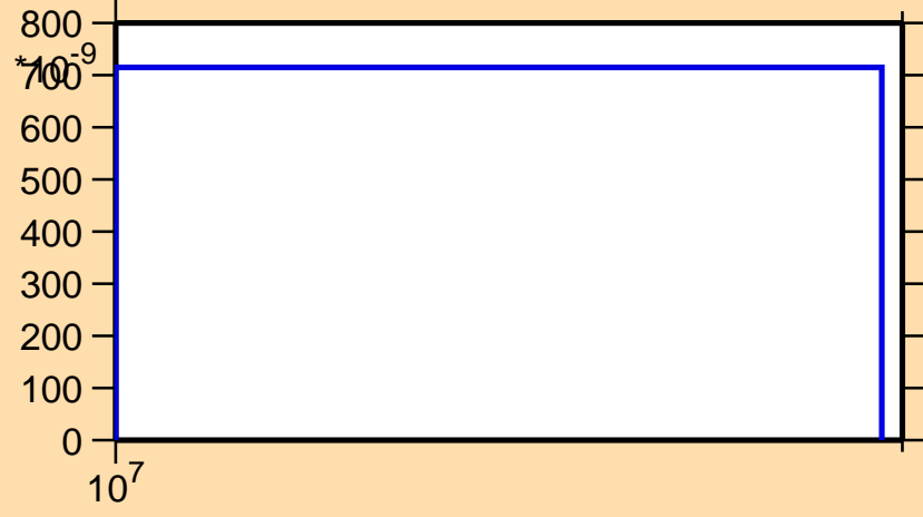
\sigma vs. E for ^{77}\text{Ga}(n,\alpha)
