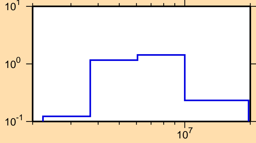
\sigma vs. E for ^{77}\text{Ga}(n,n\text{cont.})
