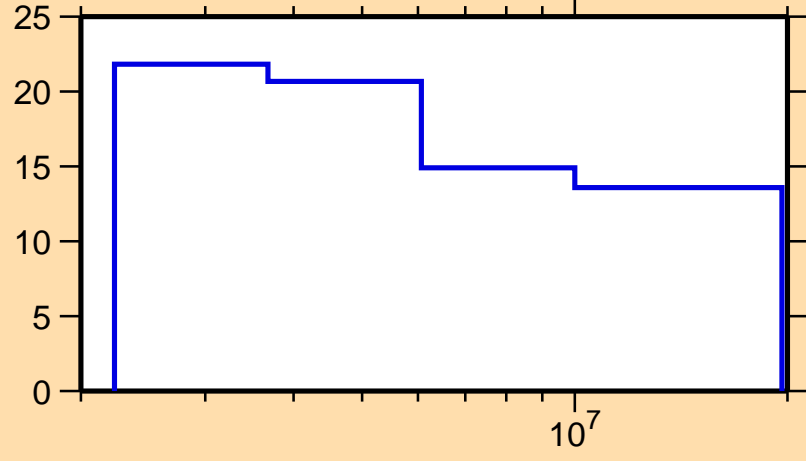
\Delta\sigma/\sigma vs. E for ^{77}\text{Ga}(n,n\text{onl.})
