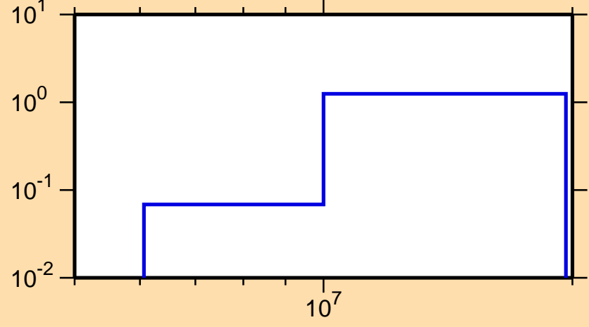
\sigma vs. E for ^{77}\text{Ga}(n,2n)
