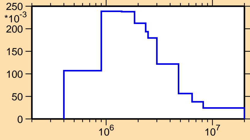
\sigma vs. E for ^{77}\text{Ga}(n,n_4)
