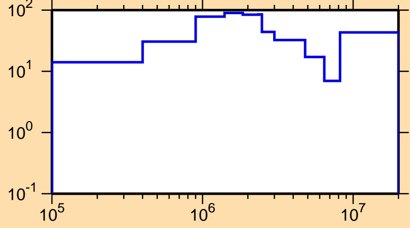
\Delta\sigma/\sigma vs. E for ^{77}\text{Ga}(n,\text{el.})
