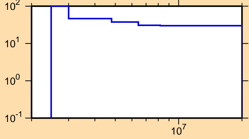
\Delta\sigma/\sigma vs. E for ^{77}\text{Ga}(n,n\text{cont.})
