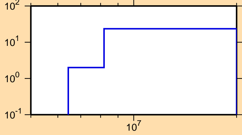
\Delta\sigma/\sigma vs. E for ^{77}\text{Ga}(n,\text{tot.})
