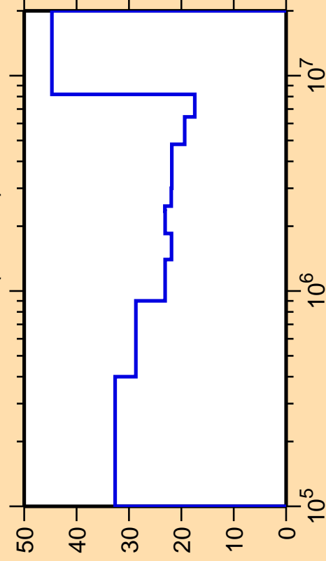
\Delta\sigma/\sigma vs. E for ^{77}\text{Ga}(n,\text{inel.})
