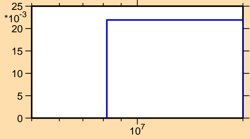
\sigma vs. E for ^{77}\text{Ga}(n,3n)
