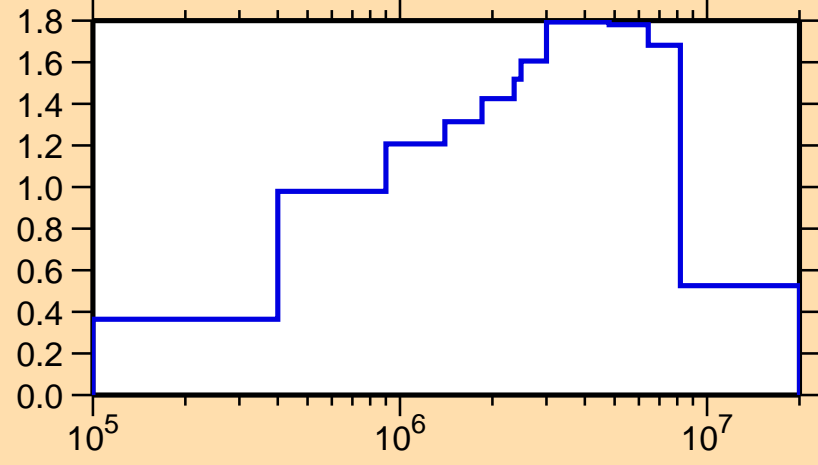
\sigma vs. E for ^{77}\text{Ga}(n,\text{inel.})
