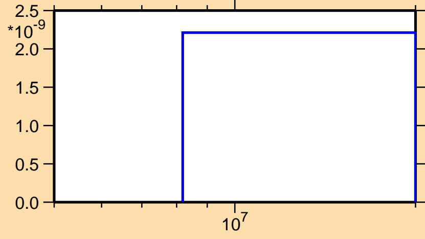
\sigma vs. E for ^{77}\text{Ga}(n,nt)
