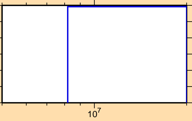
\sigma vs. E for ^{77}\text{Ga}(n,n\alpha)
