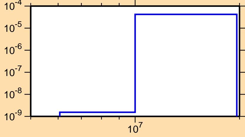
\sigma vs. E for ^{78}\text{Ga}(n,\alpha)
