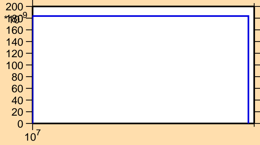
\sigma vs. E for ^{78}\text{Ga}(n,\alpha)
