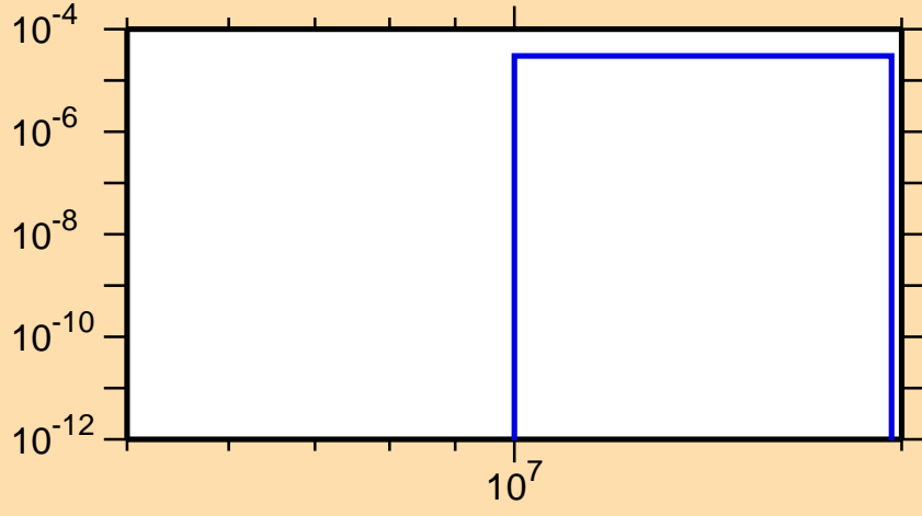
\sigma vs. E for ^{78}\text{Ga}(n,t)
