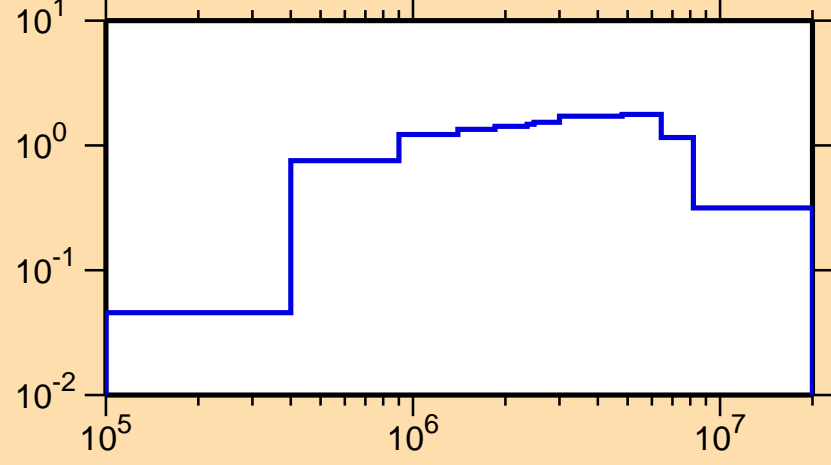
\sigma vs. E for ^{78}\text{Ga}(n,\text{inel.})
