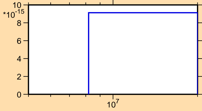
\sigma vs. E for ^{78}\text{Ga}(n,2n\alpha)
