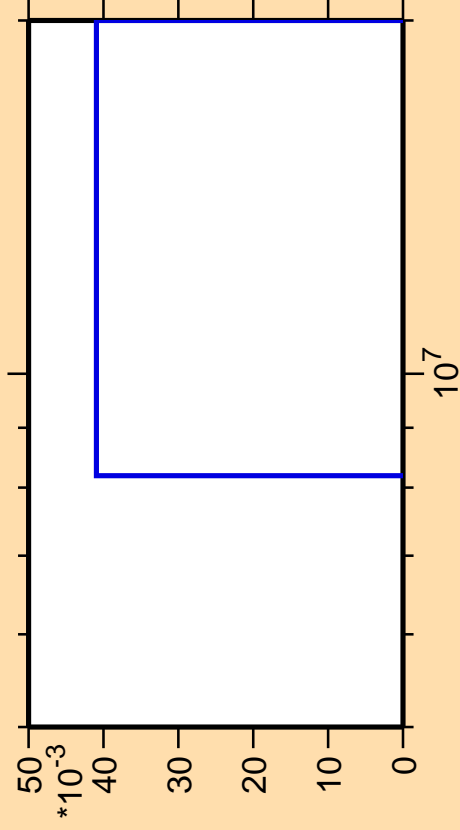
\Delta\sigma/\sigma vs. E for ^{78}\text{Ga}(n,2n\alpha)
