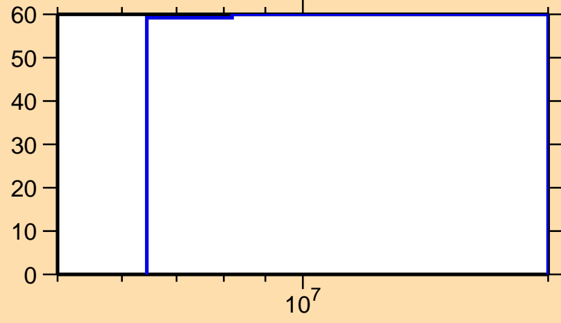
\Delta\sigma/\sigma vs. E for ^{78}\text{Ga}(n,n\text{cont.})
