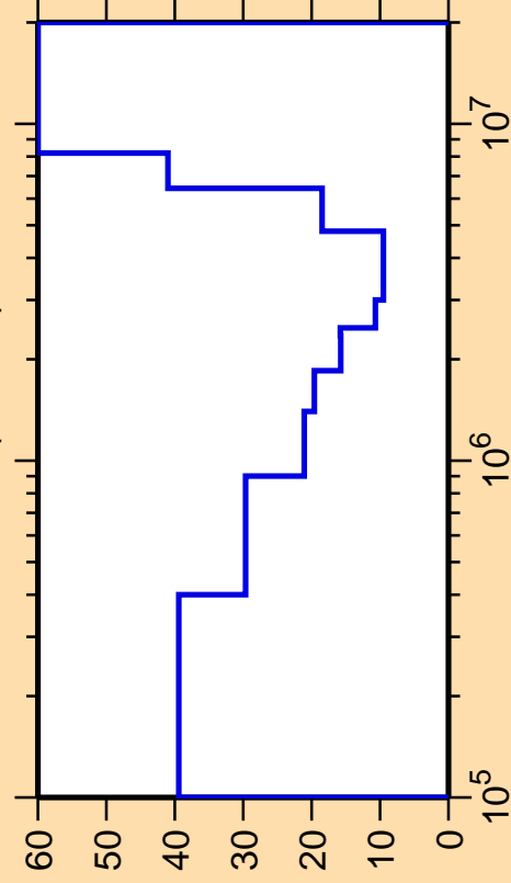
\Delta\sigma/\sigma vs. E for ^{78}\text{Ga}(n,\text{inel.})
