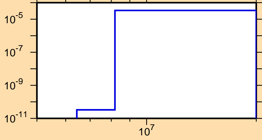
\sigma vs. E for ^{78}\text{Ga}(n,\alpha)
