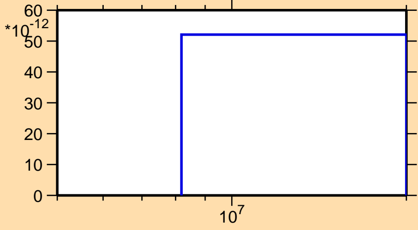
\sigma vs. E for ^{78}\text{Ga}(n,2np)
