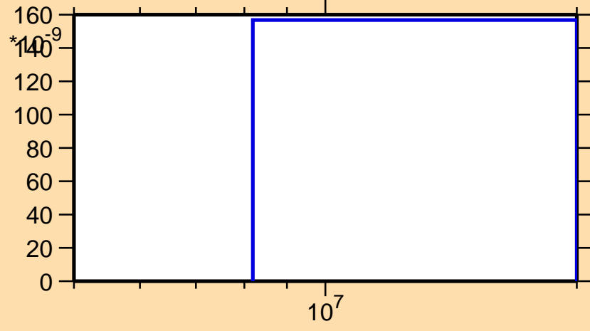
\sigma vs. E for ^{78}\text{Ga}(n,n\alpha)
