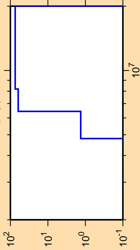
\Delta\sigma/\sigma vs. E for ^{78}\text{Ga}(n,p)
