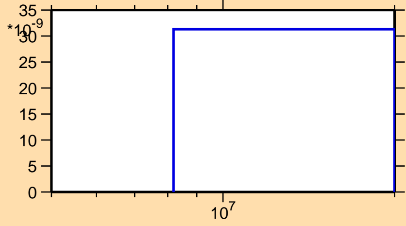
\sigma vs. E for ^{78}\text{Ga}(n,\text{nd})
