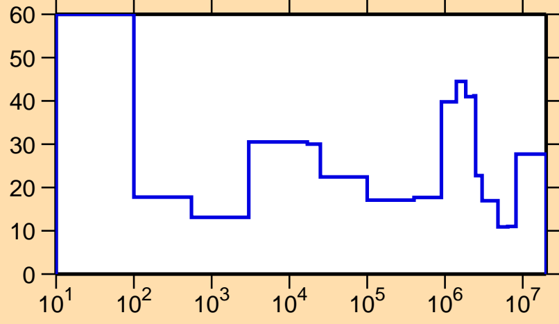
\Delta\sigma/\sigma vs. E for ^{78}\text{Ga}(n,\text{tot.})
