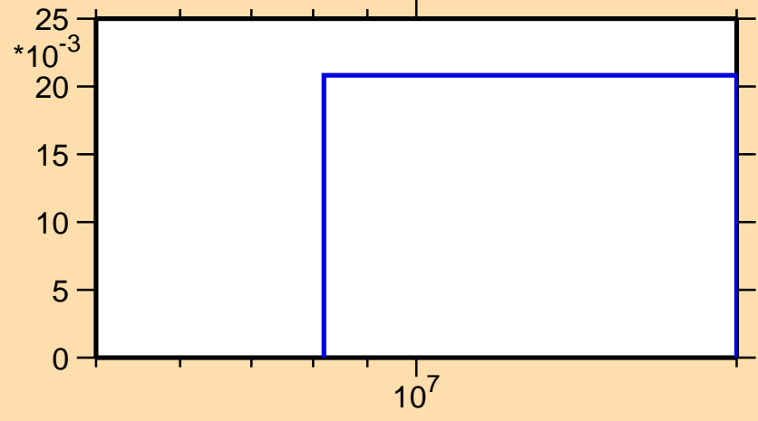
\sigma vs. E for ^{78}\text{Ga}(n,3n)
