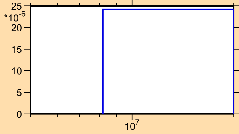
\sigma vs. E for ^{78}\text{Ga}(n,t)
