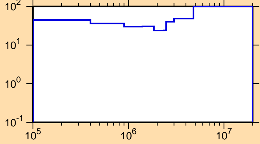
\Delta\sigma/\sigma vs. E for ^{78}\text{Ga}(n,n_1)
