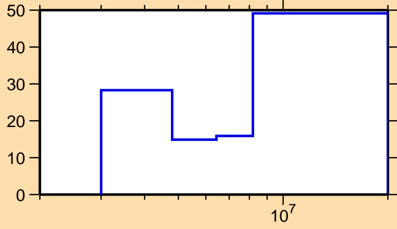
\Delta\sigma/\sigma vs. E for ^{78}\text{Ga}(n,\text{el.})
