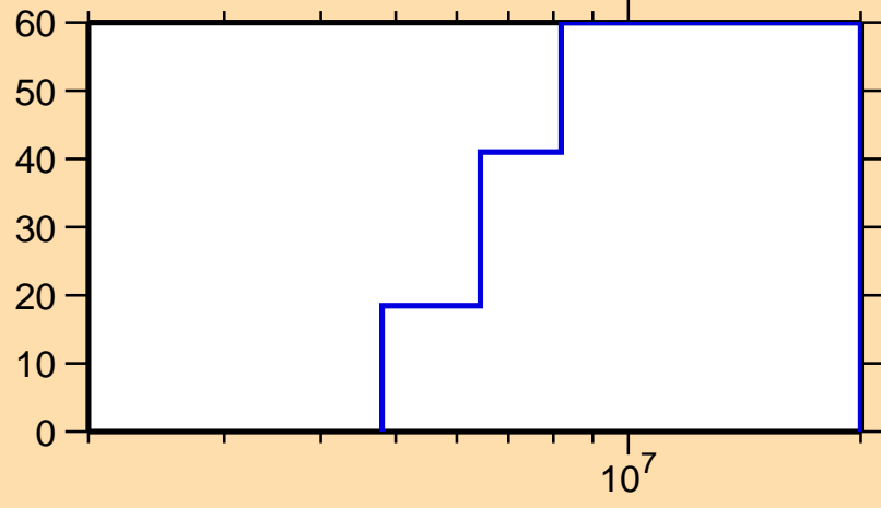
\Delta\sigma/\sigma vs. E for ^{78}\text{Ga}(n,\text{inel.})
