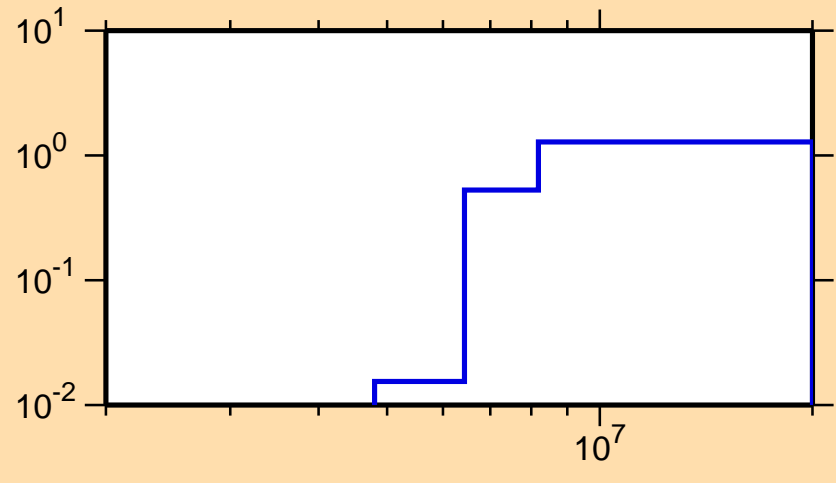
\sigma vs. E for ^{78}\text{Ga}(n,2n)
