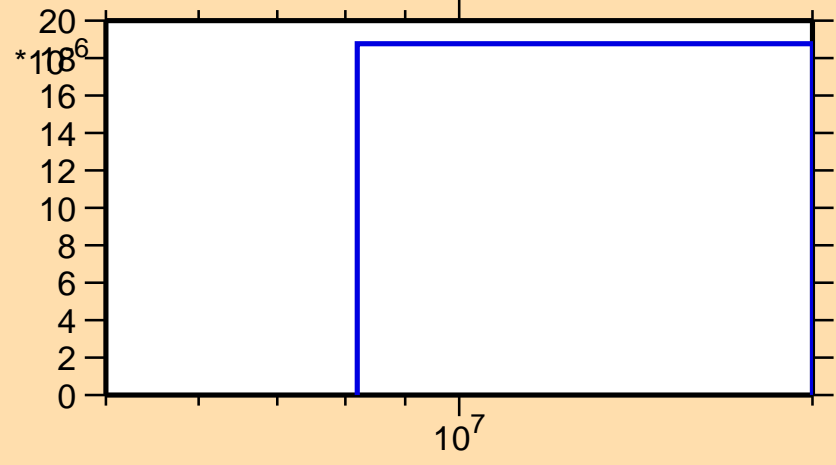
\sigma vs. E for ^{78}\text{Ga}(n,np)
