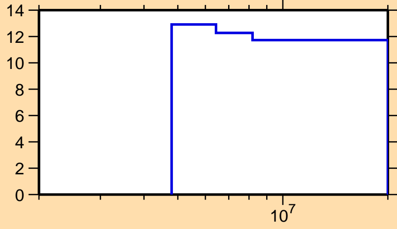
\Delta\sigma/\sigma vs. E for ^{78}\text{Ga}(n,\text{nonel.})
