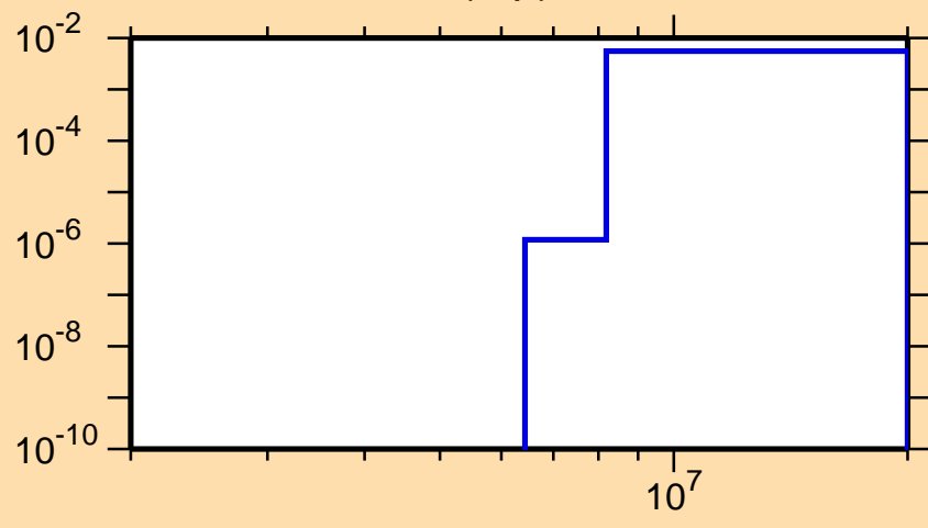
\sigma vs. E for ^{78}\text{Ga}(n,p)
