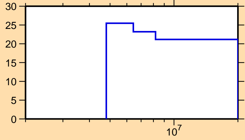
\Delta\sigma/\sigma vs. E for ^{78}\text{Ga}(n,2n)
