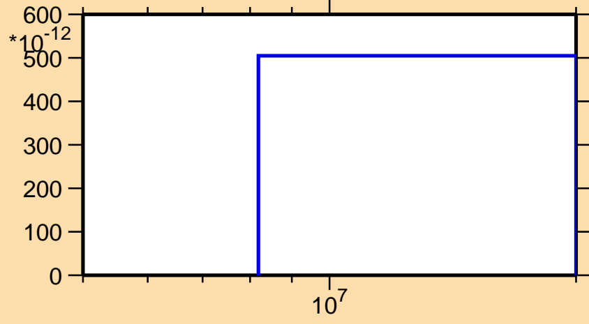
\sigma vs. E for ^{78}\text{Ga}(n,nt)
