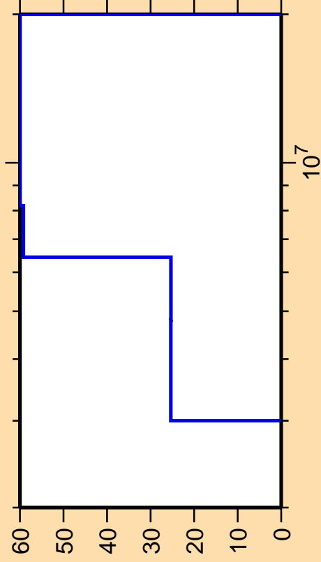
\Delta\sigma/\sigma vs. E for ^{78}\text{Ga}(n,n\text{cont.})
